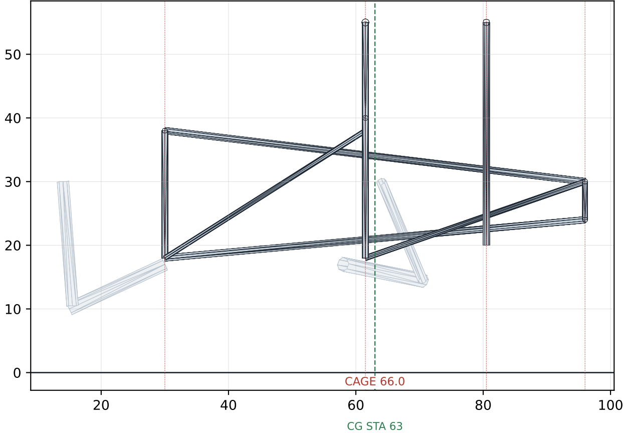
SIDE — WELDED 4130 CAGE (fabric pod removed)
