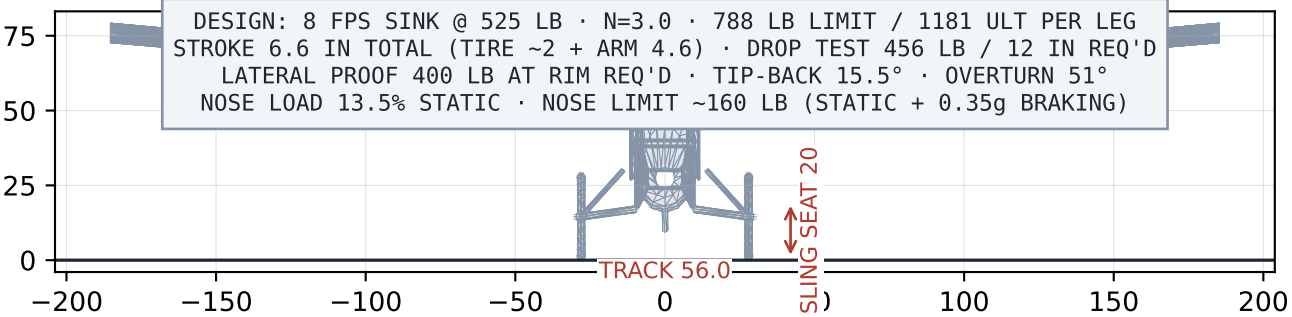
FRONT — TRACK AND STANCE
