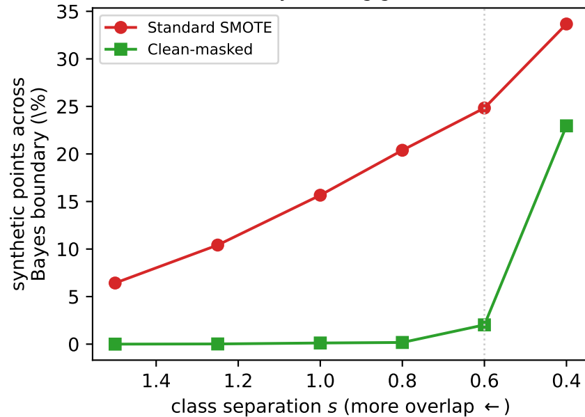
Boundary-crossing generation
