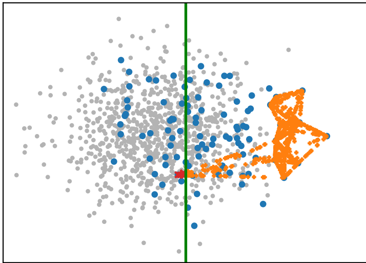
Clean-masked SMOTE
