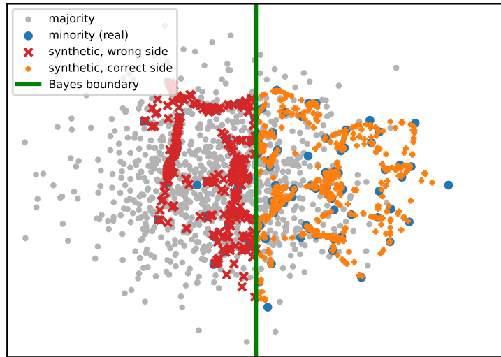
Standard SMOTE
