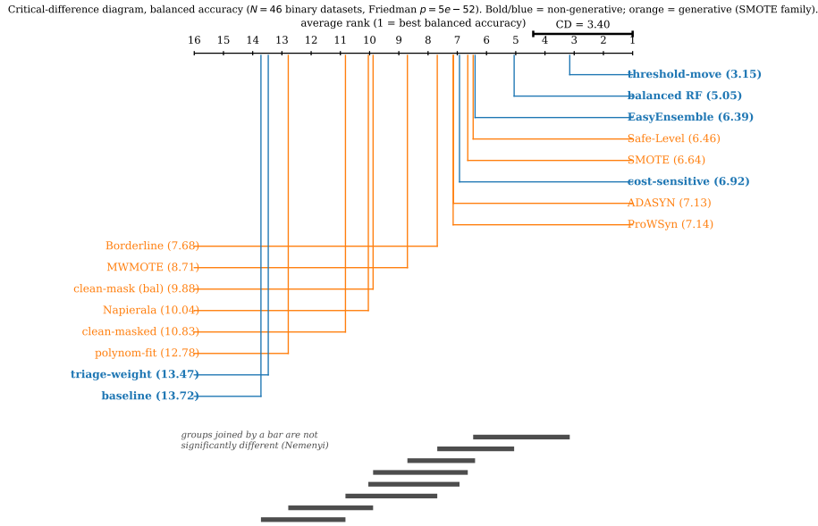
Fig. 4. Critical-difference diagram (Friedman–Nemenyi, \alpha = 0.05 , N = 46 binary datasets) of mean per-dataset balanced-accuracy rank over the full 16-strategy menu. Lower rank (right) is better. Non-generative strategies (blue) threshold-moving, balanced RF, and EasyEnsemble attain the best ranks; the SMOTE family ranks in the middle; non-rebalancing methods rank worst.
