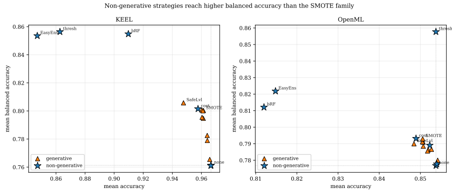
Fig. 5. Accuracy–balanced-accuracy plane per roster, at the default decision threshold . Non-generative strategies (blue \star ) reach higher balanced accuracy than the generative SMOTE family (orange \triangle ); dotted lines mark the do-nothing baseline. At threshold parity this gap largely closes (Table 4).
