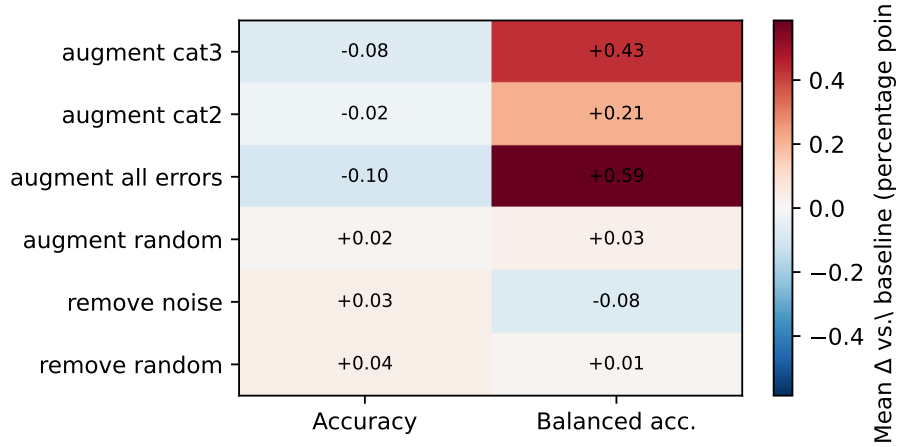
Fig. 3. Interventional validation: mean metric change vs. the no-augmentation baseline by augmentation target (50 datasets, fixed budget). Cat 3 (boundary) augmentation reproduces the SMOTE signature — balanced-accuracy gain at an accuracy cost — while random augmentation is null.
