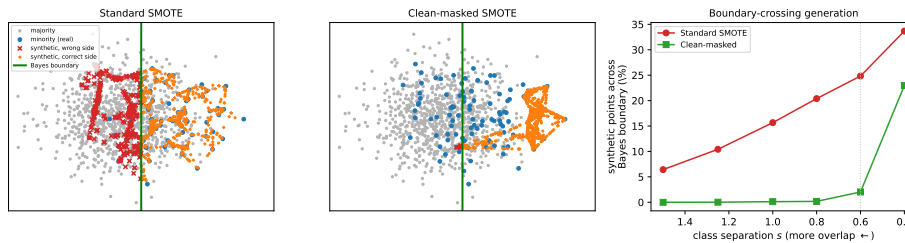
Fig. 2. Mechanism on controlled 2D Gaussians (9:1; balanced Bayes boundary x = 0 , green). Left/middle: at moderate overlap ( s = 0.6 ) standard SMOTE scatters synthetic minority points (red \times ) across the boundary into majority territory; masking the boundary seeds keeps generation on the minority side. Right: the fraction of synthetic points crossing the boundary rises with overlap for SMOTE but stays near zero when boundary seeds are excluded.
