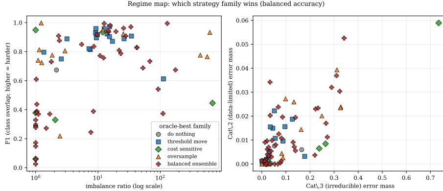
Fig. 6. Regime map: the oracle-best strategy family per dataset, over imbalance ratio vs. class overlap (F1, left) and over the triage Cat 3/Cat 2 error masses (right). Oversampling (orange) is best in a minority of regimes; balanced ensembles and threshold-moving cover most datasets.
