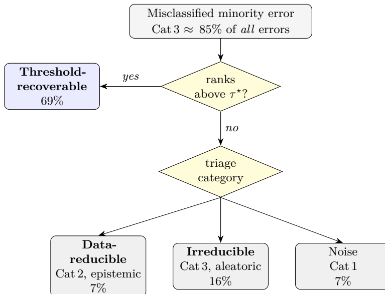
Fig. 1. How the misclassified minority filters into the three remedy classes. The decomposition asks threshold-recoverability first : an error the model already ranks above the tuned threshold \tau^* is threshold-recoverable whatever its triage category. Only the residue is split by triage into data-reducible (Cat 2), irreducible (Cat 3), or noise (Cat 1). Because most boundary (Cat 3) errors are well-ranked, the irreducible remedy class (16%) is a strict subset of Cat 3 — which is itself \sim 85\% of all errors — which is why 16\% \ll 85\% . Percentages are means over datasets (Table 2).
