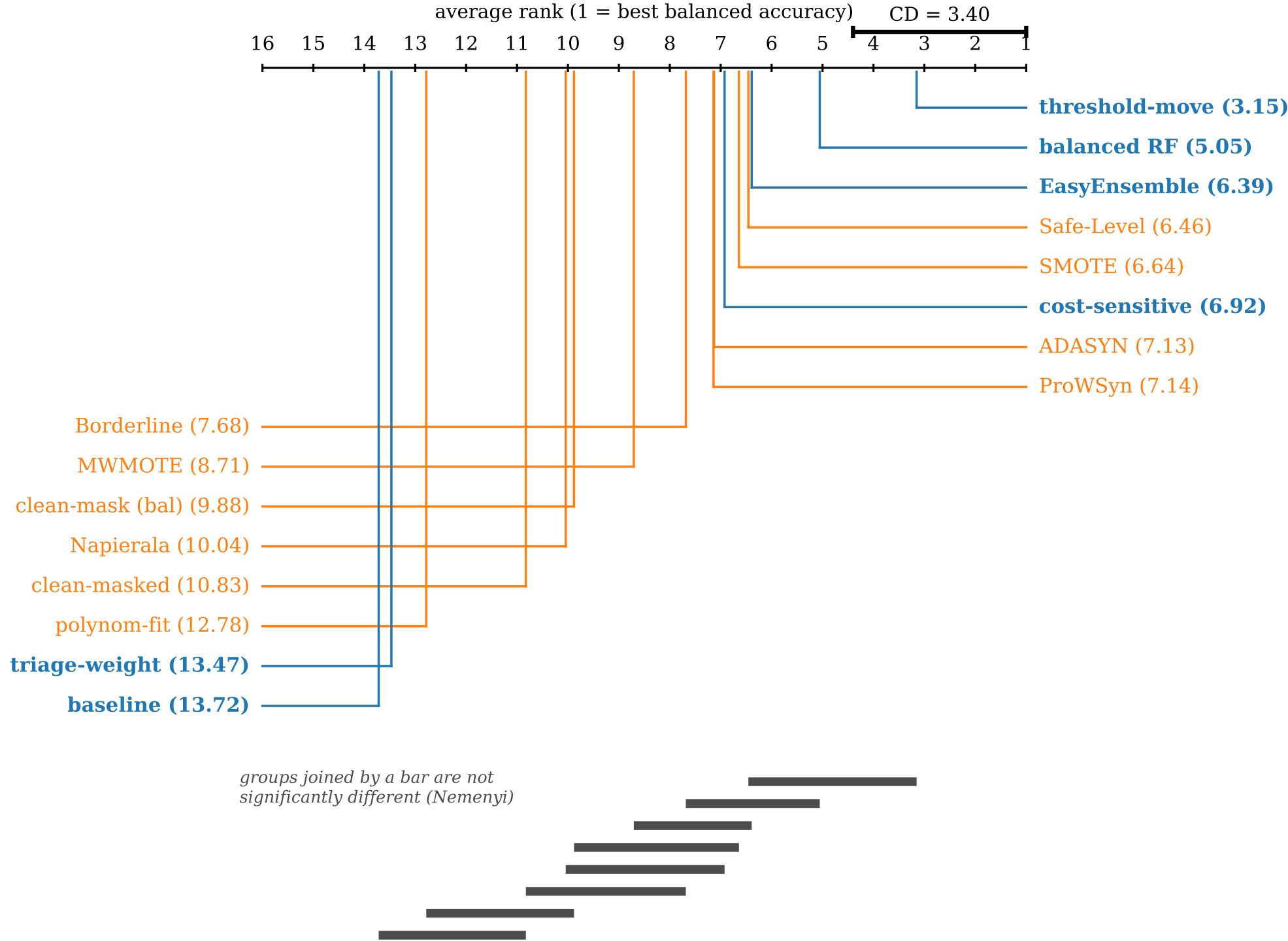
Critical-difference diagram, balanced accuracy ( N = 46 binary datasets, Friedman p = 5e - 52 ). Bold/blue = non-generative; orange = generative (SMOTE family).
