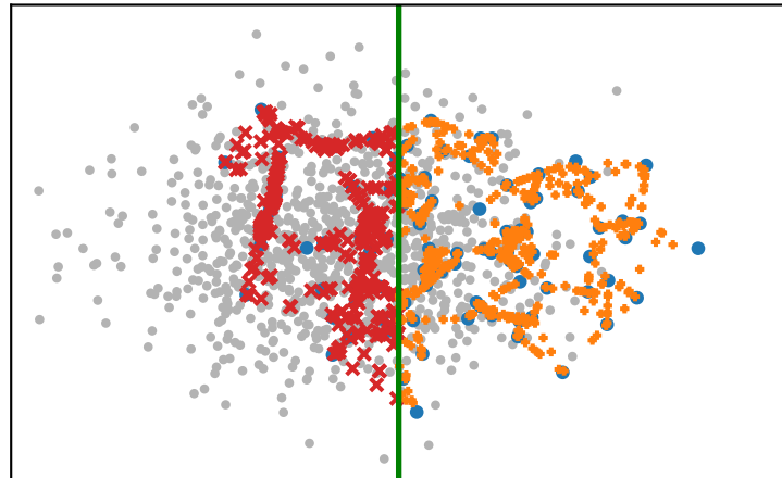
Standard SMOTE
