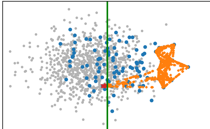
Clean-masked SMOTE
