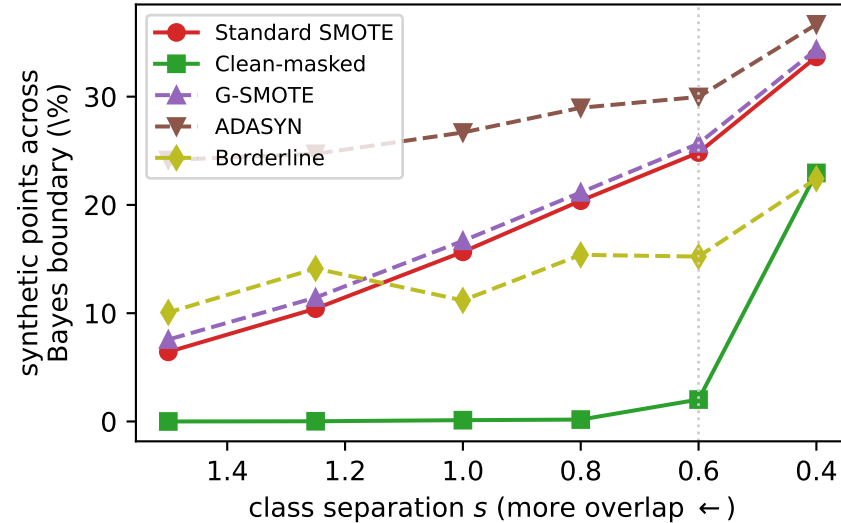
Boundary-crossing generation
