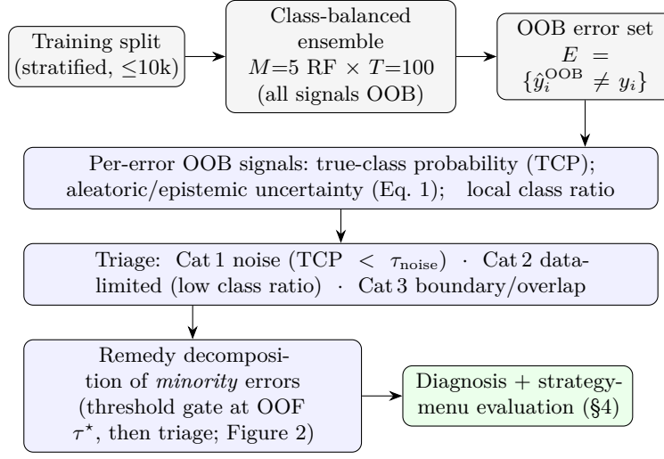
Fig. 1. End-to-end pipeline. Every model-derived signal (error set, true-class probability, uncertainty decomposition) comes from out-of-bag predictions of a class-balanced random-forest ensemble; errors are triaged into three categories; the misclassified minority is mapped to remedies via the threshold-recoverability gate of §3.3; the diagnosis is then evaluated against the 16-strategy menu.
