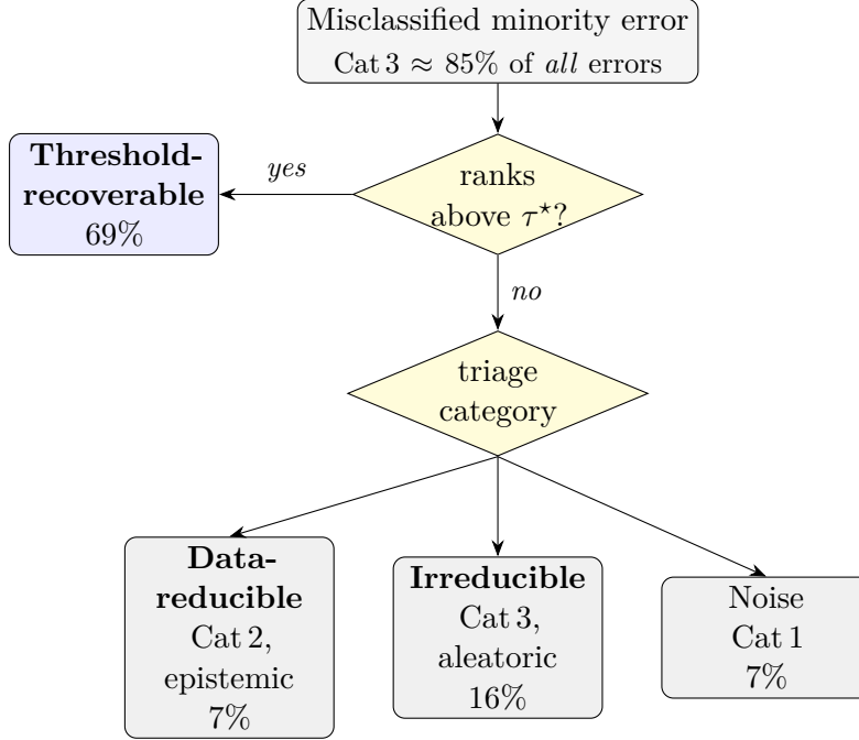
Figure 2: How the misclassified minority filters into the three remedy classes. The decomposition asks threshold-recoverability first : an error the model already ranks above the tuned threshold \tau^* is threshold-recoverable whatever its triage category. Only the residue is split by triage into data-reducible (Cat 2), irreducible (Cat 3), or noise (Cat 1). Because most boundary (Cat 3) errors are well-ranked, the irreducible remedy class (16%) is a strict subset of Cat 3 (which is itself \sim 85\% of all errors), which is why 16\% \ll 85\% . Percentages are means over datasets (Table 3).
