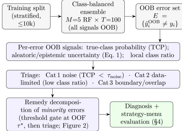
Figure 1: End-to-end pipeline. Every model-derived signal (error set, true-class probability, uncertainty decomposition) comes from out-of-bag predictions of a class-balanced random-forest ensemble; errors are triaged into three categories; the misclassified minority is mapped to remedies via the threshold-recoverability gate of §3.3; the diagnosis is then evaluated against the 16-strategy menu.
