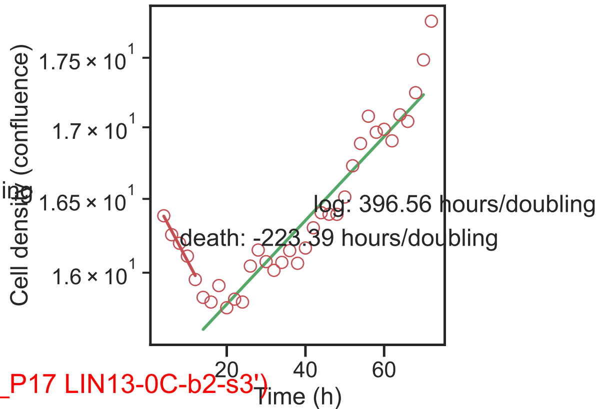
Iterative RANSAC method
