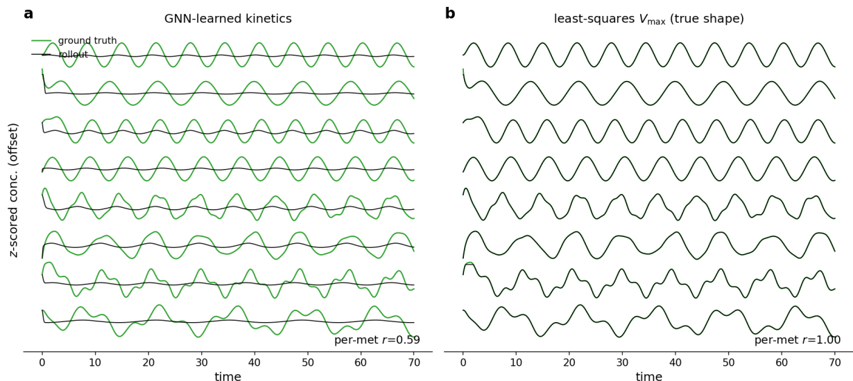
Figure 14: Right parameters give a perfect rollout; the GNN finds neither. Free rollout of the driven E. coli core network (eight highest-variance metabolites, z -scored, stacked) vs ground truth (green). (a) With the GNN-learned kinetics the rollout (black) drifts off in amplitude/phase — per-metabolite Pearson 0.59, and V_{\max} unrecovered. (b) With V_{\max} from a least-squares solve given the true substrate shape, the rollout overlays the truth exactly (per-metabolite Pearson 1.00). A single correct solution nails both parameters and rollout; the GNN’s mediocre rollout and wrong V_{\max} are two symptoms of the same shape \times scale learnability gap, not of an ill-posed problem.
