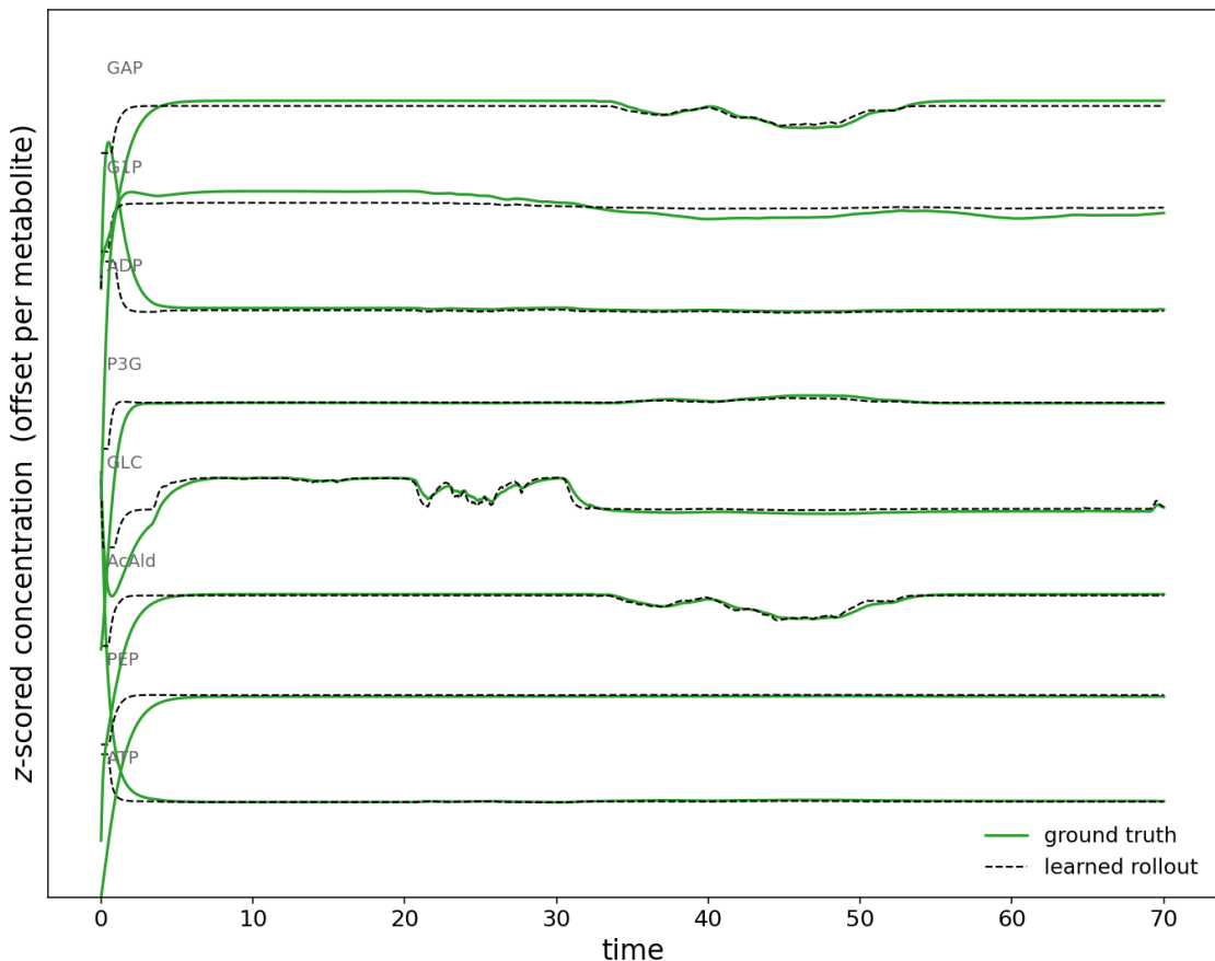
Figure 4: Rung 1 glycolysis: free-running rollout, ground truth vs learned (glyco_ar_base, stimulus supplied). The eight highest-variance metabolites, z -scored and stacked by a vertical offset: ground truth (green) vs. the learned free autoregressive rollout (dashed black). The rollout tracks the trajectory with no divergence; rollout Pearson vs. the true trajectory is 0.997 globally (0.89 per-metabolite). This is in-sample (single trajectory, no held-out run), and despite the good rollout the rate constants are not recovered ( V_{max} recovery R^2 \approx 0 , Fig. 5). Reproduced by figures/glyco_rollout.py .
