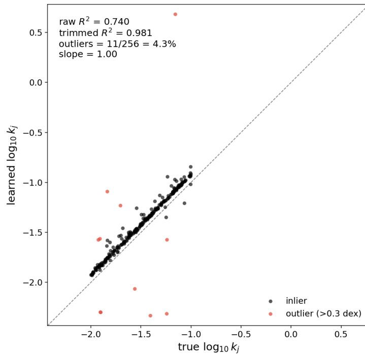
Figure 2: Toy-model rate-constant recovery (leak-free, seed 77). Learned vs. true \log_{10} k_j for all 256 reactions after the \text{MLP}_{\text{sub}} scalar ( \alpha ) correction; dashed line is identity. Inliers (black) lie on the diagonal at slope 1.00; the 11 red points (4.3%) exceed the 0.3-dex outlier threshold. Raw R^2 = 0.74 over all reactions, trimmed R^2 = 0.98 excluding outliers, within the 10%-outlier gate.
