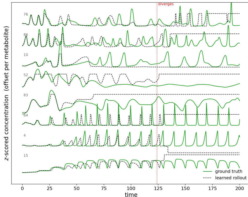
Figure 3: Toy-model free rollout (seed 77) . The eight highest-variance metabolites, z -scored and stacked by a vertical offset: ground truth (green) vs. the learned free autoregressive rollout (dashed black, clipped to its band). The rollout tracks the oscillations early and drifts with accumulating error until it diverges at time \approx 124 (red line). Rollout Pearson vs. the true trajectory: 0.96 (time < 25 ) \rightarrow 0.74 (up to divergence), then \ll 0 . The rate constants are recovered (Fig. 2) but the single-step-trained model is not a stable simulator.
