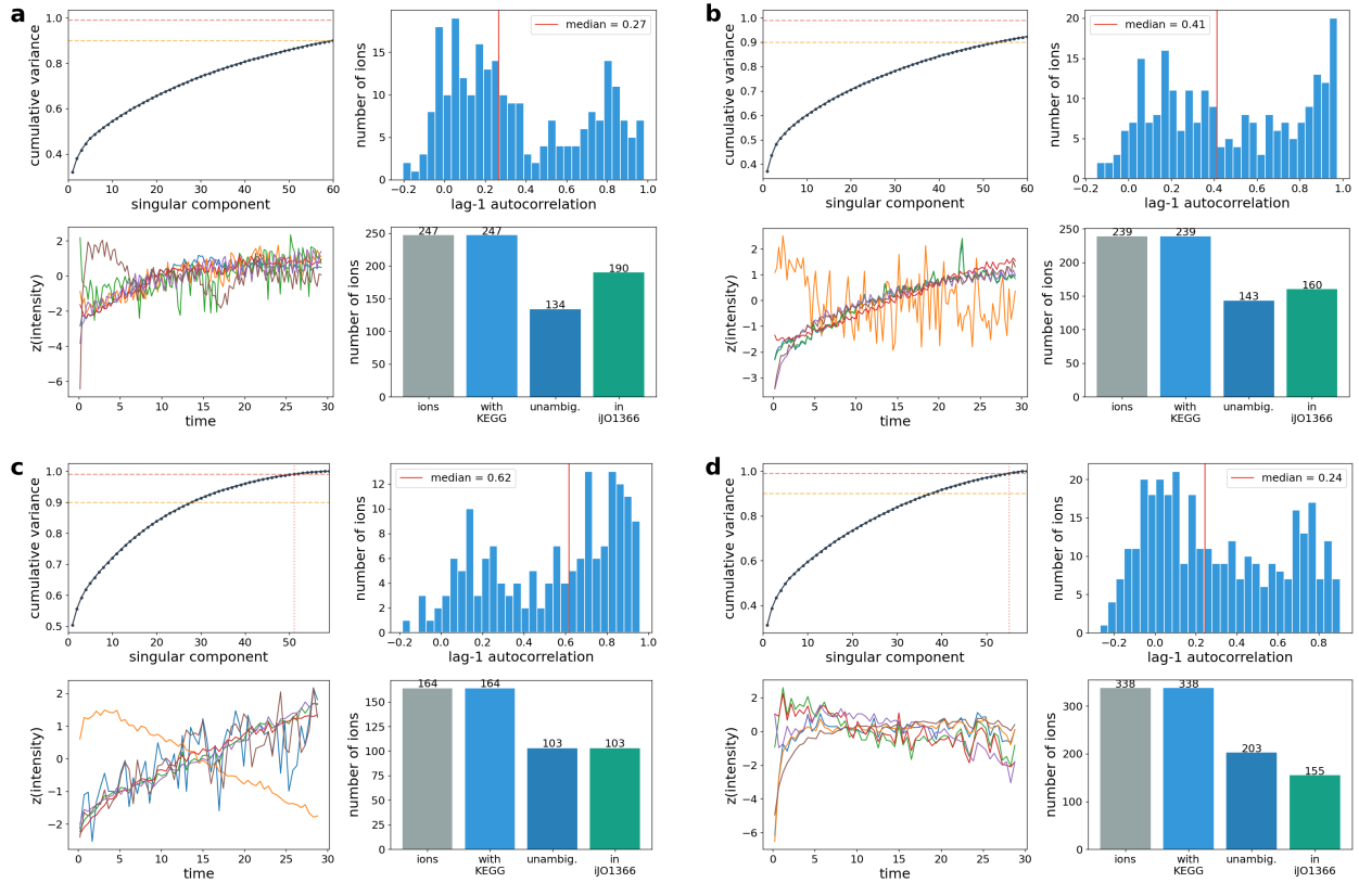
Figure 7: Identical amenability probes across the four measured datasets: (a) E. coli , (b) B. subtilis , (c) Y. lipolytica , (d) hybrid. Within each panel, top-left: SVD cumulative variance (low-rank); top-right: per-ion lag-1 autocorrelation; bottom-left: six highest-variance traces ( z -scored); bottom-right: KEGG coverage against iJO1366. Low-rank structure and network coverage recur in all four; only Y. lipolytica shows smooth, slowly varying traces and a right-shifted autocorrelation distribution.
