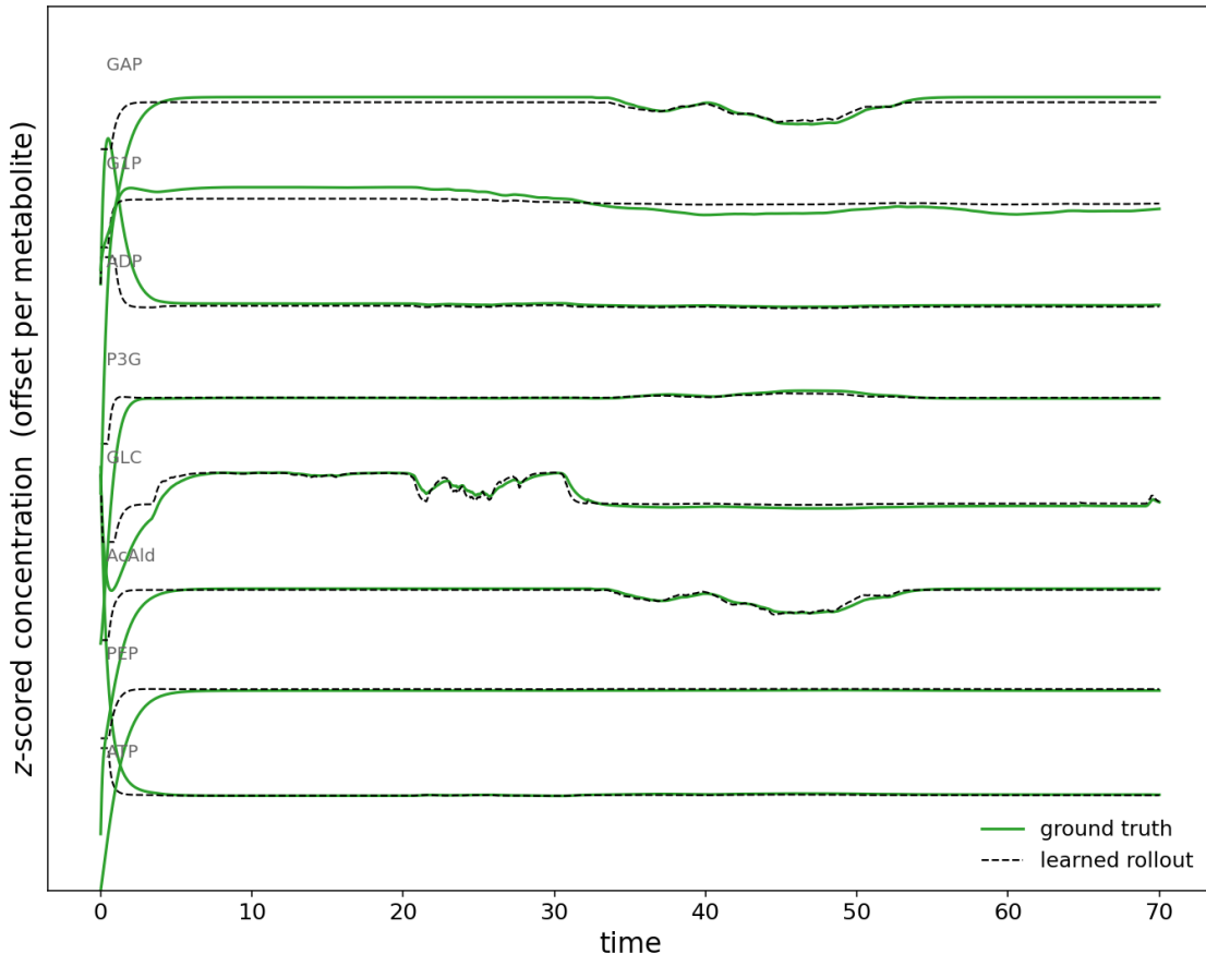
Figure 4: Rung 1 glycolysis: free-running rollout, ground truth vs learned (the curriculum model, stimulus supplied). The eight highest-variance metabolites, z-scored and stacked by a vertical offset: ground truth (green) vs. the learned free autoregressive rollout (dashed black). The rollout tracks the trajectory with no divergence; rollout Pearson vs. the true trajectory is 0.997 globally (0.89 per-metabolite). This is in-sample (single trajectory, no held-out run), and despite the good rollout the rate constants are not recovered ( V_{max} recovery R^2 \approx 0 , Fig. 5).
