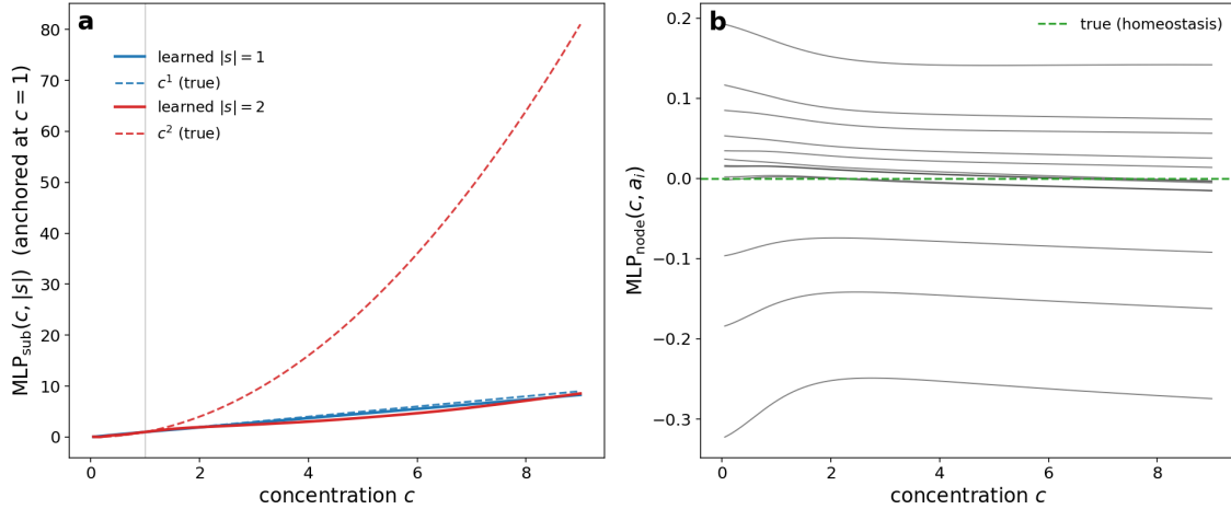
Figure 1: Toy model: the two learned functions vs. ground truth. (a) \text{MLP}_{\text{sub}}(c, |s|) (solid) vs. the true power law c^{|s|} (dashed) for |s|=1, 2 , anchored at c=1 — the substrate law is recovered. (b) \text{MLP}_{\text{node}}(c, a_i) per metabolite (the homeostasis term); it stays \approx 0 (dashed: the true zero homeostasis of this regime).
