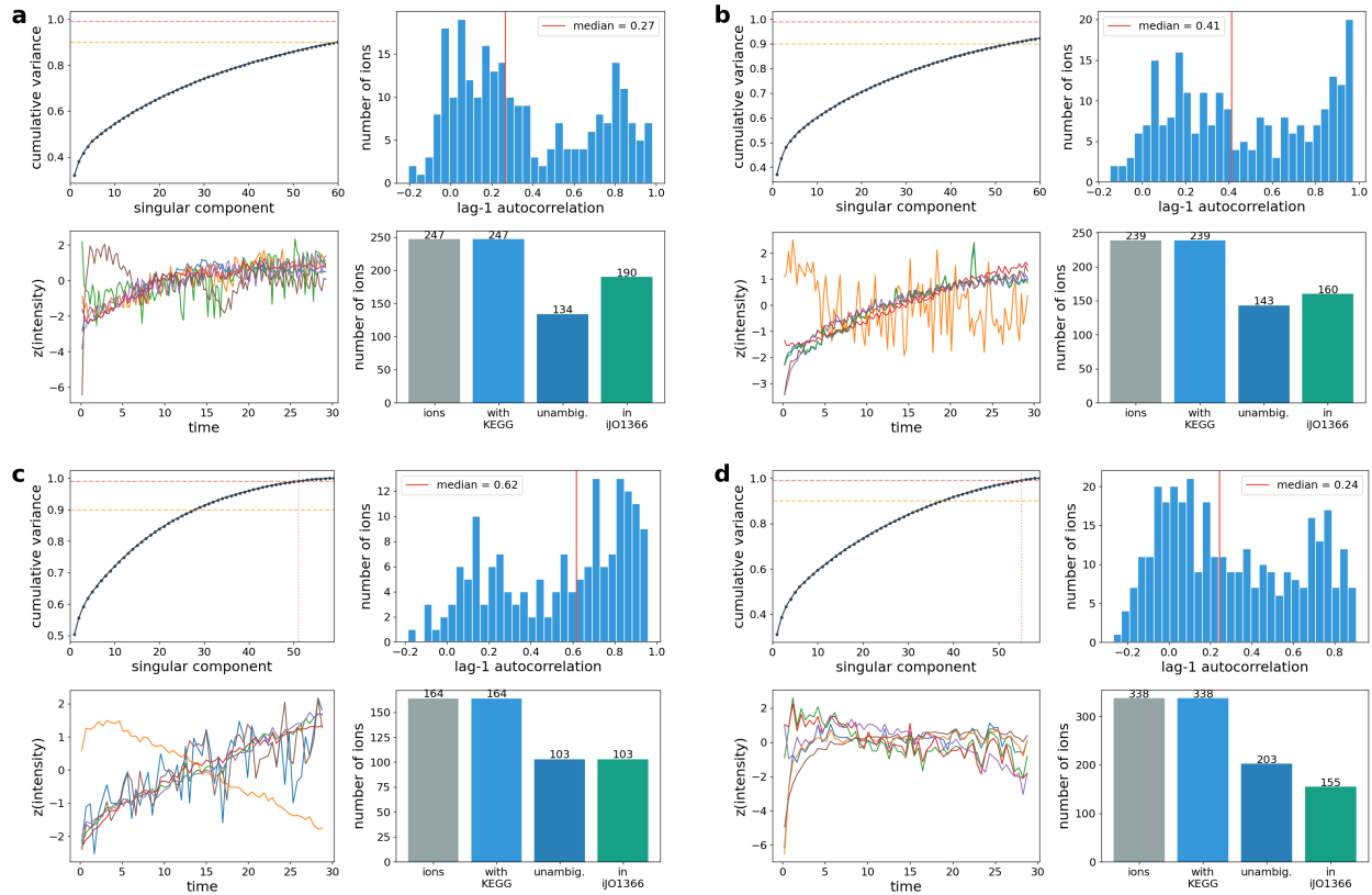
Figure 12: Identical amenability probes across the four measured datasets: (a) E. coli , (b) B. subtilis , (c) Y. lipolytica , (d) hybrid. Within each panel, top-left: SVD cumulative variance (low-rank); top-right: per-ion lag-1 autocorrelation; bottom-left: six highest-variance traces ( z -scored); bottom-right: KEGG coverage against iJO1366. Low-rank structure and network coverage recur in all four; only Y. lipolytica shows smooth, slowly varying traces and a right-shifted autocorrelation distribution.
