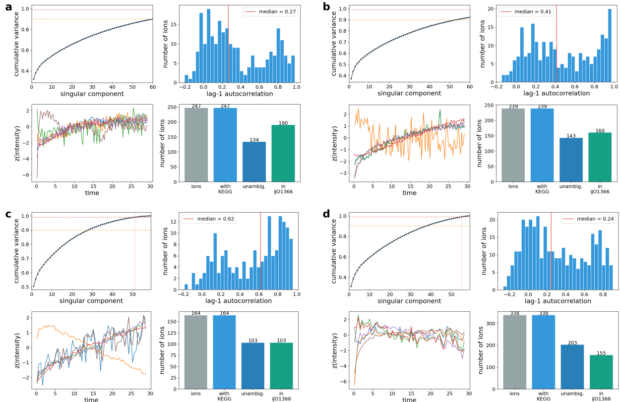
Figure 2: Identical amenability probes across the four measured datasets: (a) E. coli , (b) B. subtilis , (c) Y. lipolytica , (d) hybrid. Within each panel, top-left: SVD cumulative variance (low-rank); top-right: per-ion lag-1 autocorrelation; bottom-left: six highest-variance traces ( z -scored); bottom-right: KEGG coverage against iJ01366. Low-rank structure and network coverage recur in all four; only Y. lipolytica shows smooth, slowly varying traces and a right-shifted autocorrelation distribution. Reproduced by figures/amenability.py.
