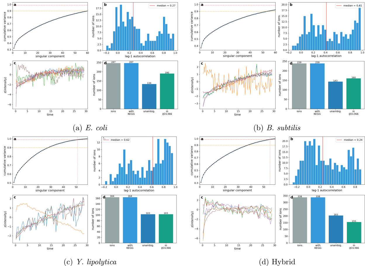
Figure 2: Identical amenability probes across the four measured datasets (each panel: (a) SVD low-rank, (b) lag-1 autocorrelation, (c) highest-variance traces, (d) iJO1366 coverage). Low-rank structure and network coverage recur everywhere; only Y. lipolytica (c) shows smooth, slowly varying traces and a right-shifted autocorrelation distribution. Reproduced by figures/amenability.py .
