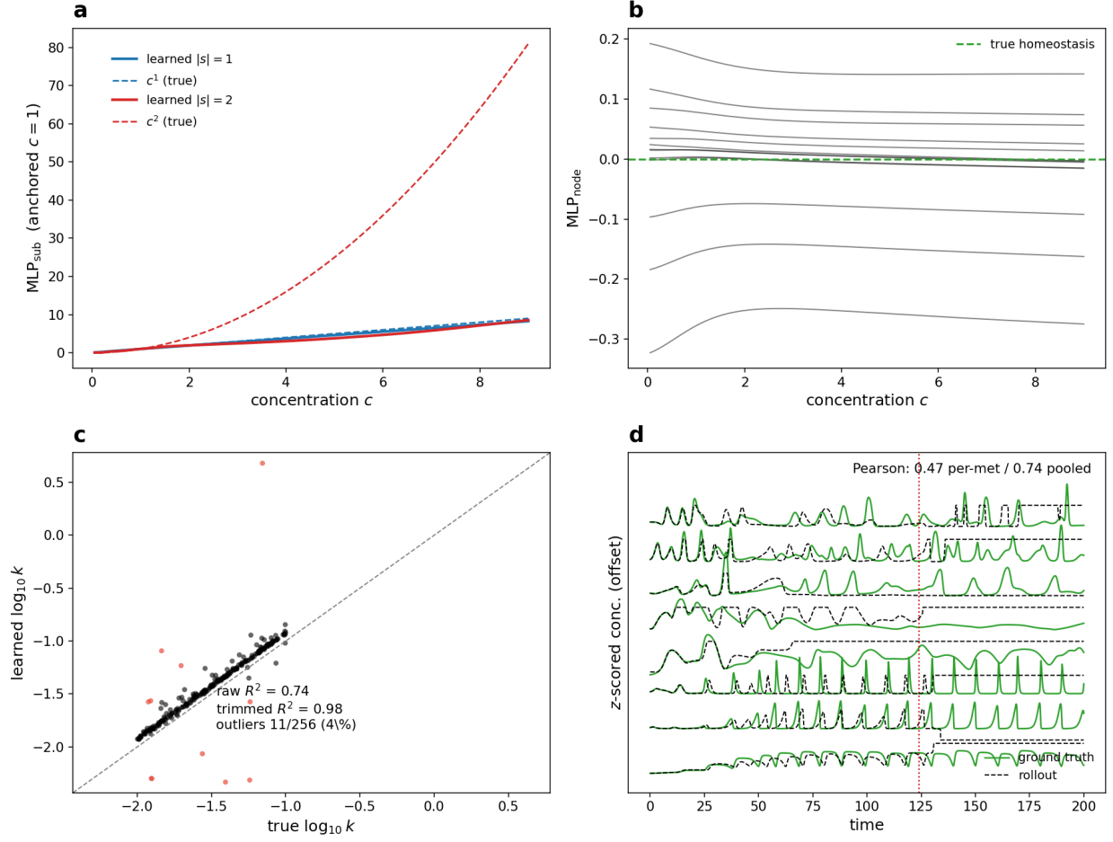
Figure 1: Toy-model results dashboard (leak-free, seed 77). (a) \text{MLP}_{\text{sub}}(c, |s|) (solid) vs. the true power law c^{|s|} (dashed) for |s|=1, 2 , anchored at c=1 : the substrate law is recovered for |s|=1 (the regime the toy contains), while the |s|=2 curve is an out-of-support extrapolation. (b) \text{MLP}_{\text{node}} per metabolite (homeostasis); it stays \approx 0 (dashed: the true zero homeostasis of this regime). (c) Rate-constant recovery: learned vs. true \log_{10} k_j for all 256 reactions after the \text{MLP}_{\text{sub}} scalar correction (dashed: identity, slope 1.00); 11 red points (4.3%) exceed the 0.3-dex outlier gate, raw R^2=0.74 , trimmed R^2=0.98 . (d) Free rollout of the eight highest-variance metabolites, z-scored and stacked: ground truth (green) vs. the learned autoregressive rollout (dashed black). It tracks the oscillations early and drifts until it diverges at time \approx 124 (red line); convergent-window rollout Pearson 0.47 per metabolite (0.74 pooled). Rate constants are recovered, but the single-step-trained model is not a stable simulator.
