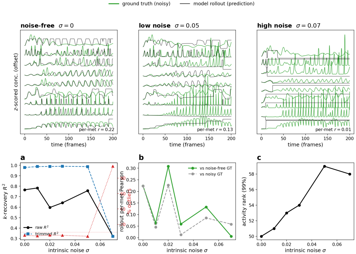
Figure 5: Companion to Fig. 1: intrinsic-noise sweep. Process noise \sigma injected into the toy generator (an SDE forcing term); single-step training on the noisy trajectory, evaluated against the noise-free twin (same network/seed). Top row: free rollout at three noise levels (noise-free, low, high) — the ground truth (green) it is scored against grows visibly noisier with \sigma , while the model’s prediction (black) stays smooth; it recovers the deterministic dynamics it never observed cleanly, but full-window per-metabolite fidelity stays modest and breaks down once the trajectory itself is corrupted ( \sigma = 0.07 ). (a) k -recovery vs. \sigma : trimmed R^2 (blue) holds at \approx 0.98 with 5–6% outliers (red) for \sigma \leq 0.05 , then collapses at \sigma = 0.07 (95% outliers); raw R^2 (black) stays within the seed-variation band. (b) Rollout per-metabolite Pearson vs. \sigma , against the noise-free GT (green) and the noisy GT (gray). (c) Activity rank vs. \sigma : the injected noise does diversify the data (35 \rightarrow 47), but on this S -given toy that diversity is not needed to identify k .
