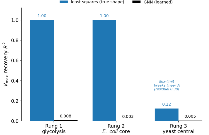
Figure 16: Least squares recovers V_{\max} ; the GNN does not (yet). V_{\max} recovery R^2 on the realistic OU-stimulus data, least squares given the true shape (blue) vs the trained GNN (black), per rung. Where the dynamics are genuinely linear in V_{\max} (rungs 1–2, reconstruction residual \sim 10^{-4} ) least squares is exact ( R^2=1.00 ) while the GNN sits at \approx 0 . Rung 3’s flux clamping invalidates the linear design matrix (residual 0.30), so even least squares degrades — a simulator artefact, not a data limit. The achievable solution exists and is easy to compute; the open problem is getting the GNN to find it.
