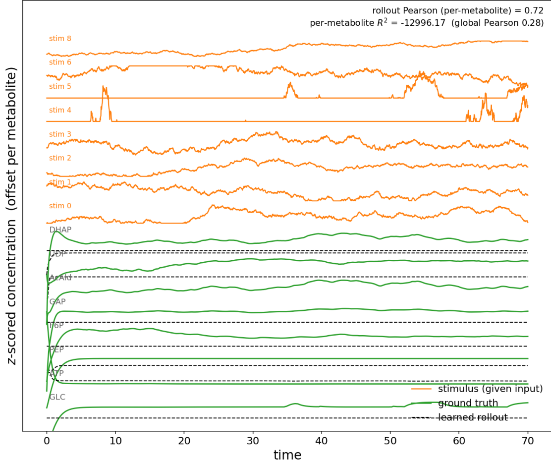
Figure 4: Rung 1 glycolysis: the held-out generalisation test. The same trained model rolled out on an unseen trajectory — a different given stimulus (orange, top) and a different initial state, comparable rank — never used in training. Unlike the in-sample case (Fig. 3), the learned rollout (dashed black) settles to the wrong levels and no longer tracks ground truth (green): global Pearson falls from 0.997 to 0.28 (global R^2 0.99 \rightarrow 0.05 ; per-metabolite R^2 strongly negative). The in-sample fit was memorisation of one trajectory, not a learned mechanism — direct evidence for the degeneracy implied by the failed V_{\max} recovery.
