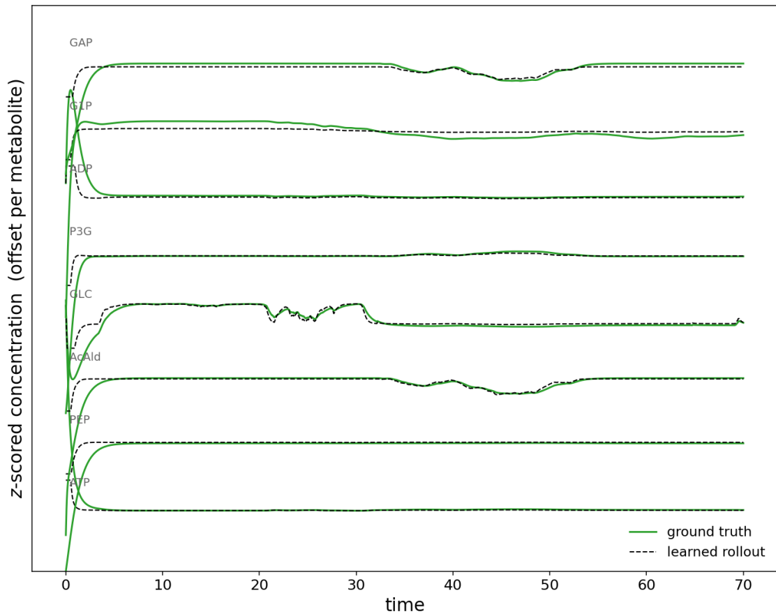
Figure 3: Rung 1 glycolysis: free-running rollout, ground truth vs learned (the curriculum model, stimulus supplied). The eight highest-variance metabolites, z -scored and stacked by a vertical offset: ground truth (green) vs. the learned free autoregressive rollout (dashed black). The rollout tracks the trajectory with no divergence; rollout Pearson vs. the true trajectory is 0.997 globally (0.89 per-metabolite). This is in-sample (single trajectory, no held-out run), and despite the good rollout the rate constants are not recovered ( V_{\max} recovery R^2 \approx 0 , Fig. 4).
