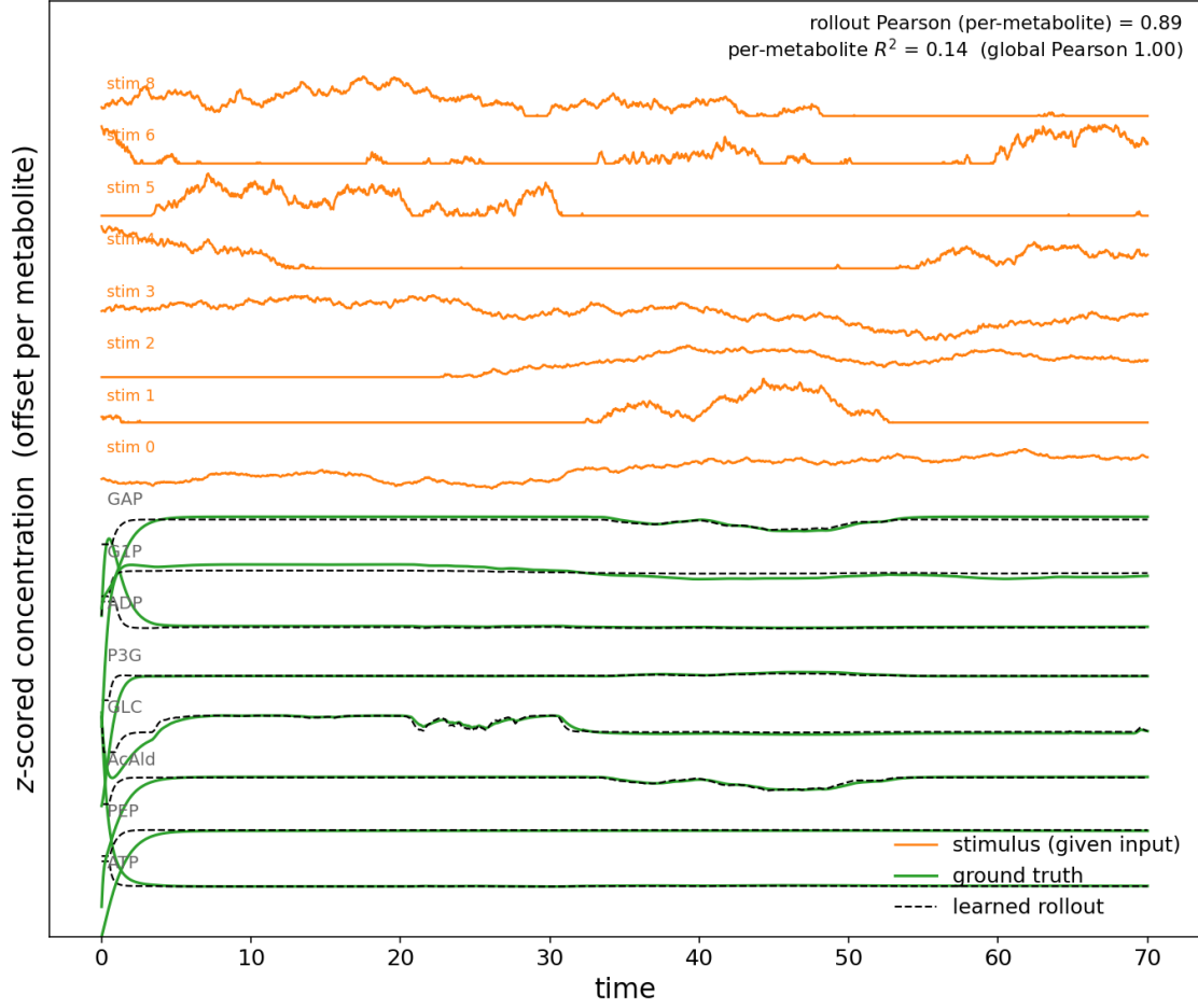
Figure 4: Rung 1 glycolysis: free-running rollout, ground truth vs learned (the curriculum model, stimulus supplied). The eight highest-variance metabolites, z -scored and stacked by a vertical offset: ground truth (green) vs. the learned free autoregressive rollout (dashed black); the nine given external stimulus channels (orange, top) are the known boundary drive supplied to the rollout, not predicted. The rollout tracks the trajectory with no divergence; rollout Pearson vs. the true trajectory is 0.997 globally (0.89 per-metabolite). But note the metabolites mostly relax to a steady state under the strong given drive — so the high Pearson is partly stimulus-driven settling, and per-metabolite R^2 is only 0.14 (the settled levels drift). This is in-sample (single trajectory, no held-out run), and despite the good-looking rollout the rate constants are not recovered ( V_{\max} recovery R^2 \approx 0 , Fig. 6).
