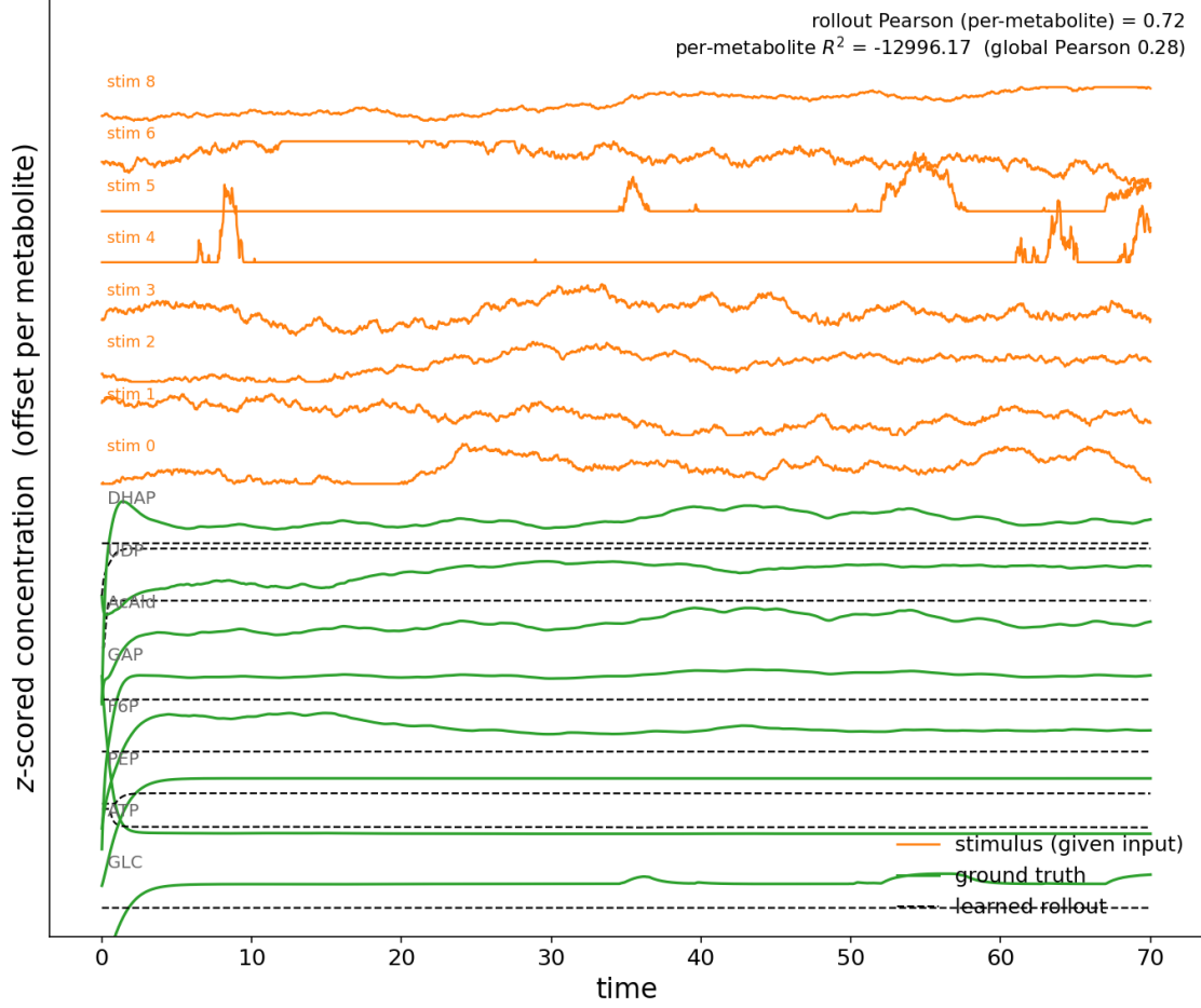
Figure 5: Rung 1 glycolysis: the held-out generalisation test. The same trained model rolled out on an unseen trajectory — a different given stimulus (orange, top) and a different initial state, comparable rank — never used in training. Unlike the in-sample case (Fig. 4), the learned rollout (dashed black) settles to the wrong levels and no longer tracks ground truth (green): global Pearson falls from 0.997 to 0.28 (global R^2 0.99 \rightarrow 0.05 ; per-metabolite R^2 strongly negative). The in-sample fit was memorisation of one trajectory, not a learned mechanism — direct evidence for the degeneracy implied by the failed V_{\max} recovery.
