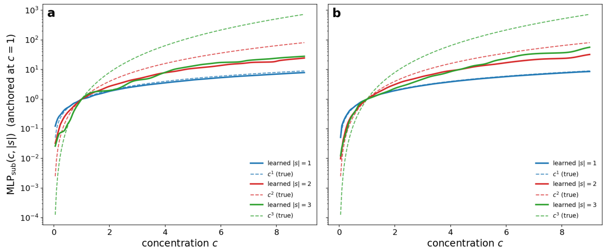
Figure 7: Curvature recovery on a regime with |s| \geq 2 (the |s| \geq 2 regime). Learned \text{MLP}_{\text{sub}}(c, |s|) (solid) vs the true power law c^{|s|} (dashed) for |s|=1, 2, 3 , log y -axis, anchored at c=1 . (a) plain MLP, (b) log-space MLP. Both track c^1 ; both bend upward for c^2, c^3 now that the data contains such reactions, with log-space bending more — but both fall well short of the true c^2 (and far short of c^3 ).
