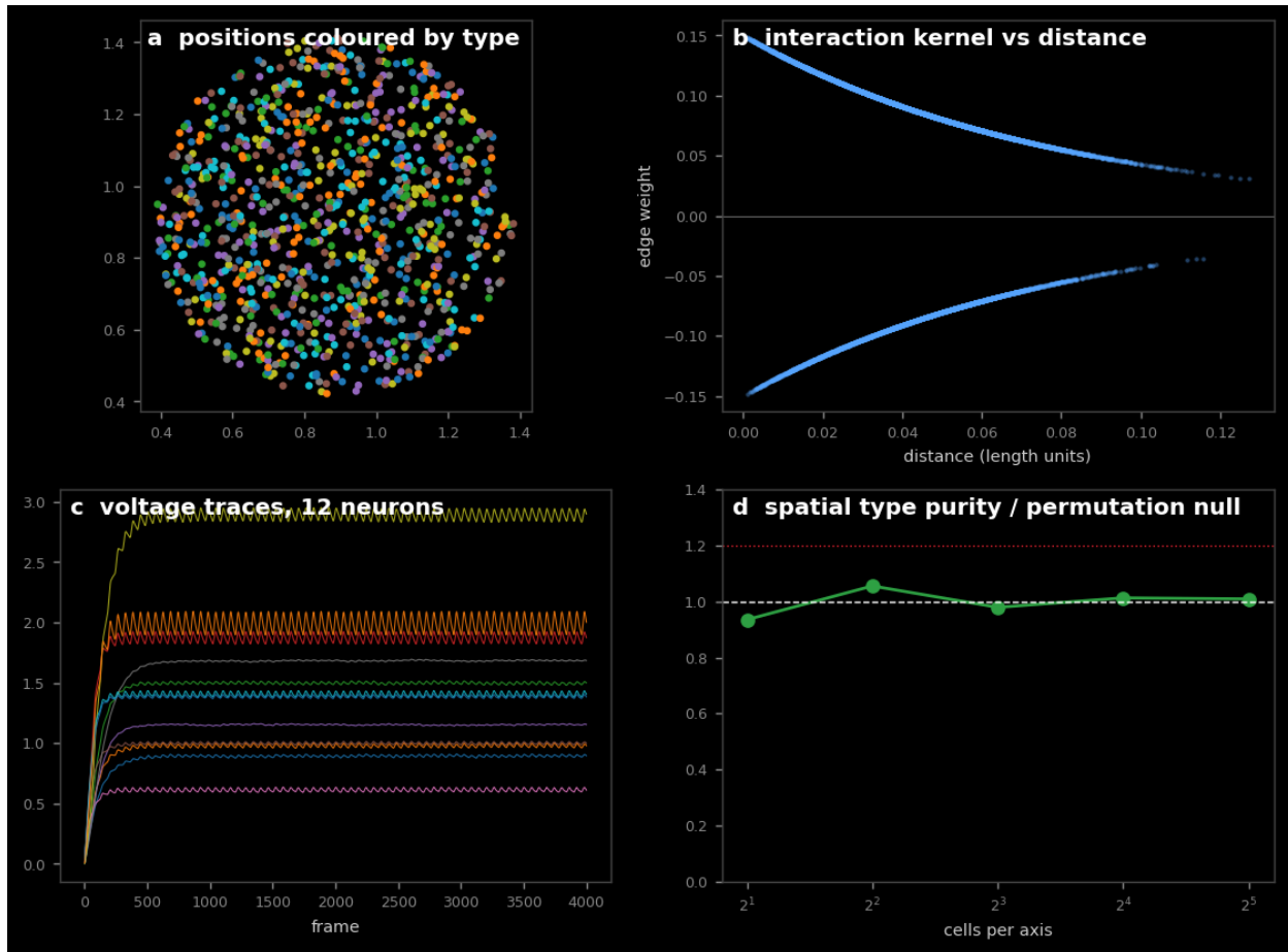
Figure 4: G16 — types are spatially mixed by construction. Threshold: spatial-cell type purity within 20% of chance ( 1/n\_types ). Measured: 1.056. Outcome: PASS.
