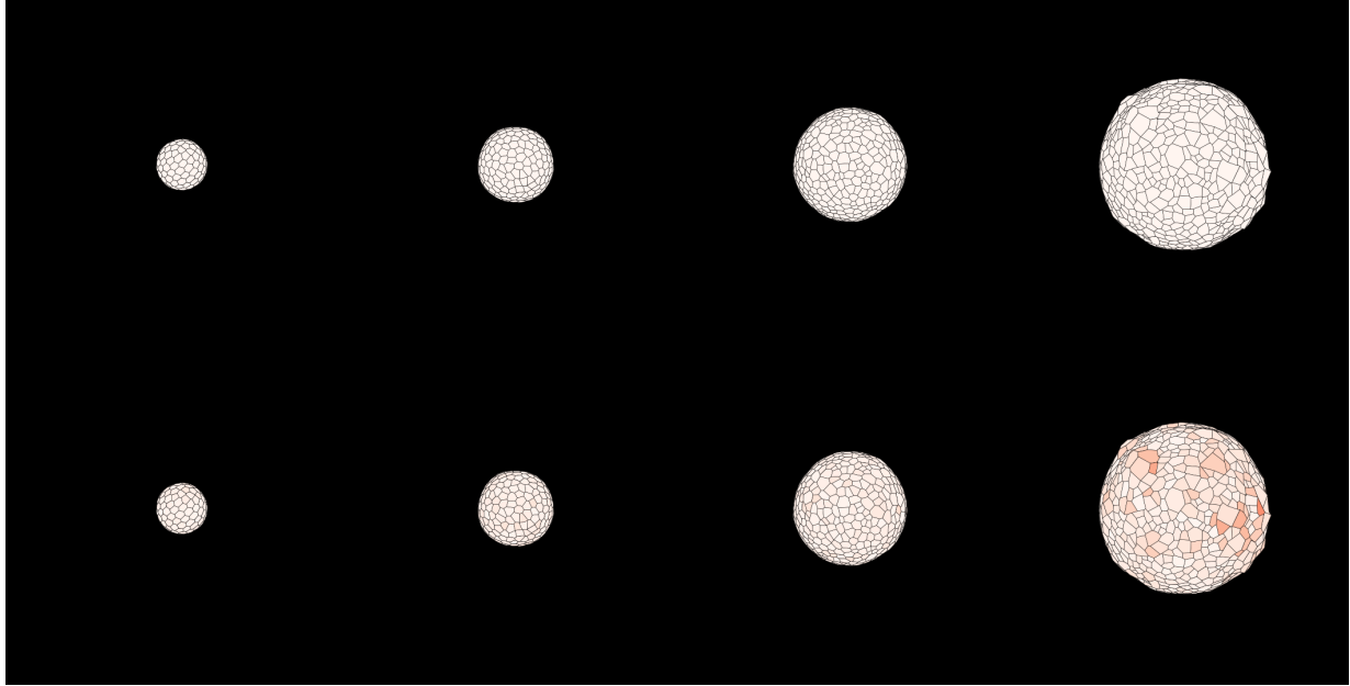
Figure 12: With aligned recording the dividing vesicle is a smooth sphere — the “hollow buckling” was a diagnostic artefact. The same physics that scored \sim 97\% “hollow” under mismatched position/topology recording strides ( posf = 151, hist = 76 at 300 frames) scores hollow \leq 0.003 once the two are recorded on the same stride ( vesicle_grow_divide_400f , 150 \rightarrow 949 cells; top row white render, bottom row coloured by the hollow flag). The “defect” lived entirely in the diagnostic’s frame pairing; the one real residue is a mild cell- area spread from the deterministic cell cycle.
