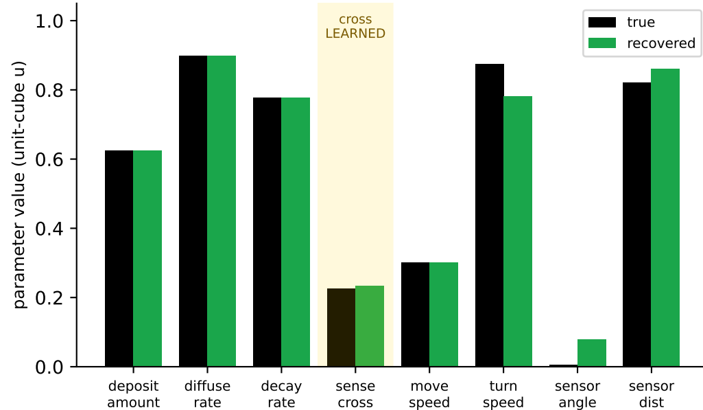
(b) four-type slime (cross now LEARNED)
