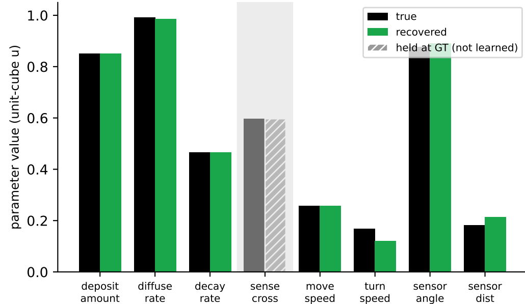
(a) full recovery -- field loss + position loss (cross HELD at GT, not learned: single-type)
