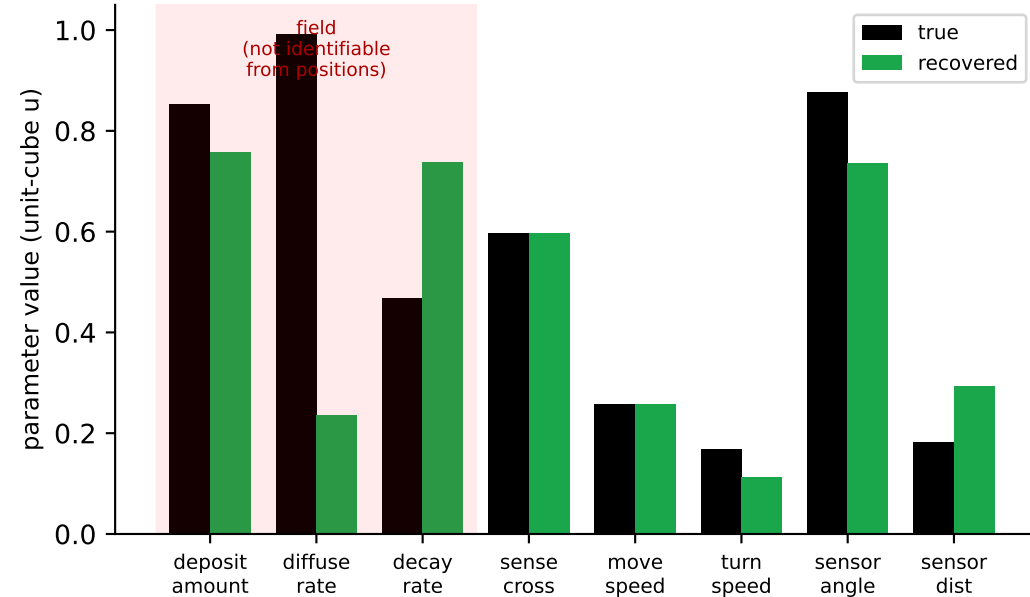
(c) POSITION-ONLY loss, no field loss (field unobserved: field params fail)
