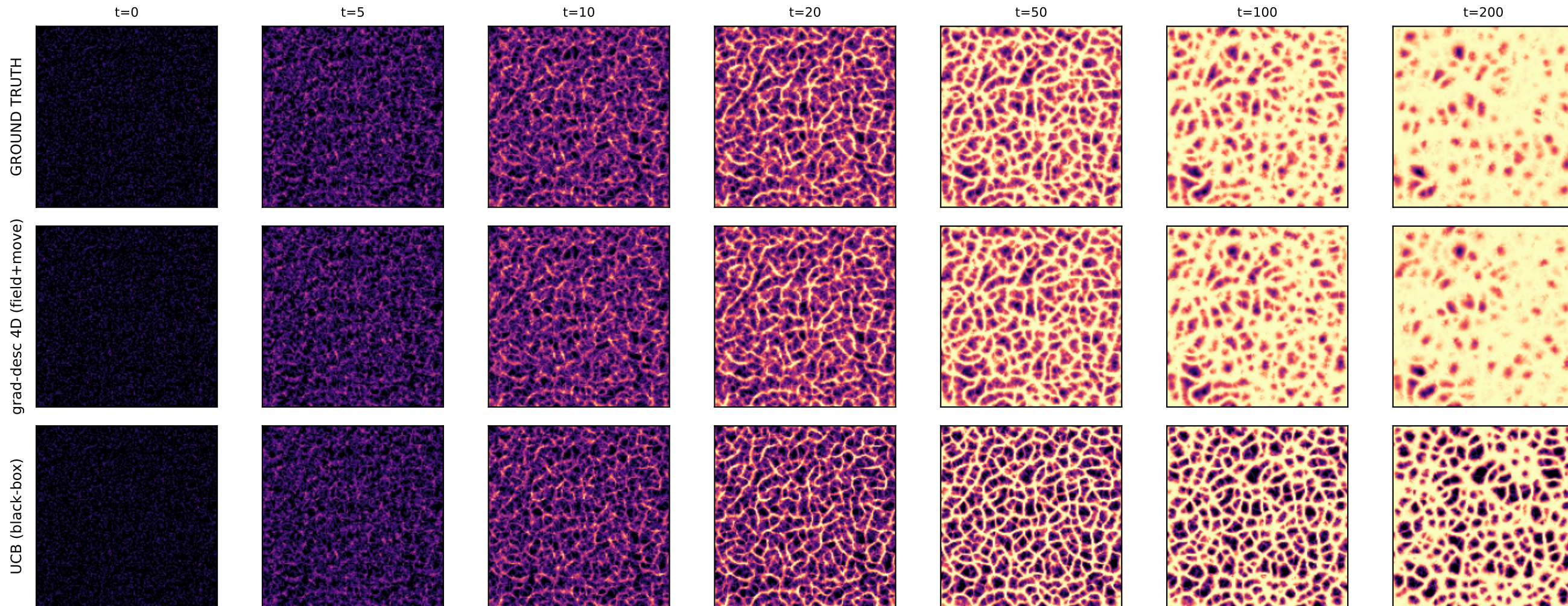
Showcase target -- chemical field evolution (baselines)
