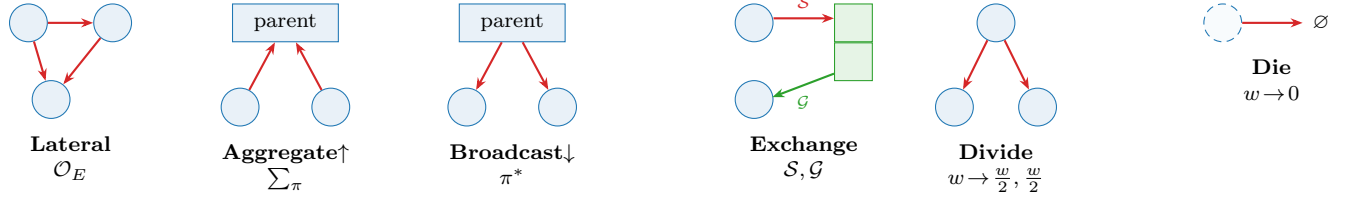
Figure 2: The six operators. The first four move state along a fixed structure: Lateral acts within a set; Aggregate and Broadcast move across containment \pi ; Exchange scatters ( \mathcal{S} ) to and gathers ( \mathcal{G} ) from a field (P2G/G2P and the metabolite–reaction graph are both Exchange). Divide and Die are structural : they change a set’s membership — cell division and death — carried on a fixed buffer by a per-element occupancy mass w .
