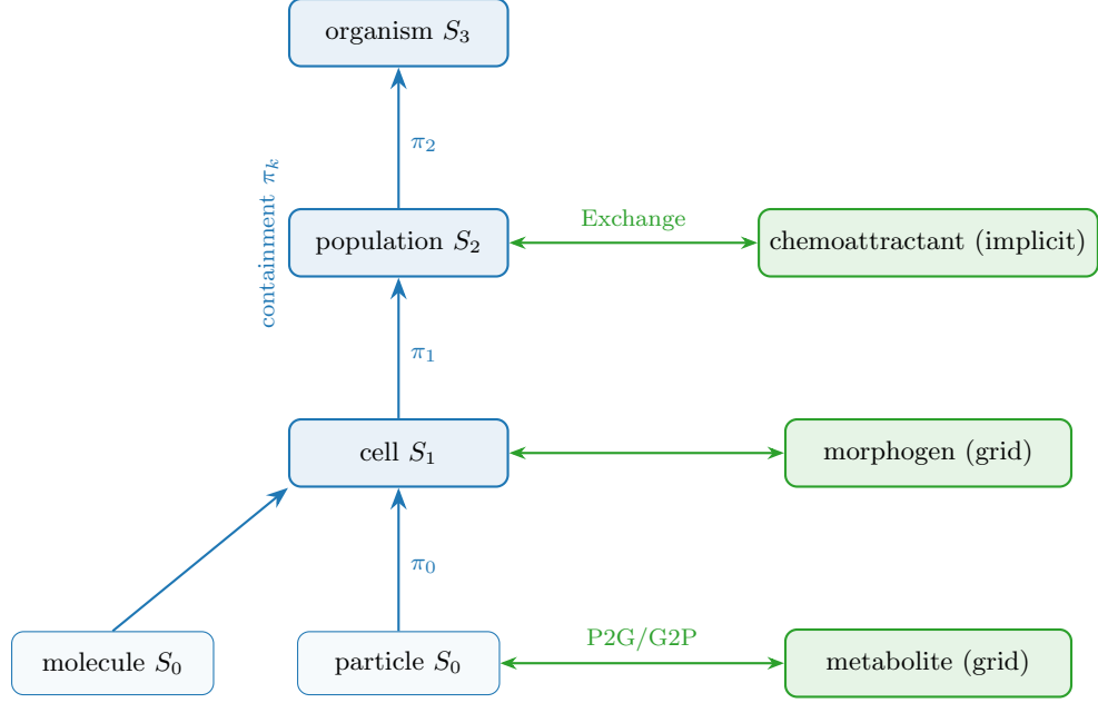
Figure 1: The container. Blue : sets on a single containment spine, linked bottom-up by the partition maps \pi_k (a cell is the set of its particles; molecules are a second leaf of the cell). Green : fields — a flat collection, each on its own grid, each bound by a bidirectional Exchange relation to the one level it couples to (drawn at that level’s height). No field nests inside the hierarchy.
