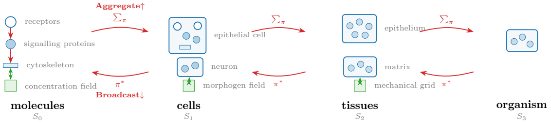
Figure 1: The hierarchy. Each level holds several distinct sets (blue) and may carry its own fields (green); operators (red) act between entities within a level, and exactly two families cross a level — Aggregate, \Sigma\pi , and Broadcast, \pi^* .
