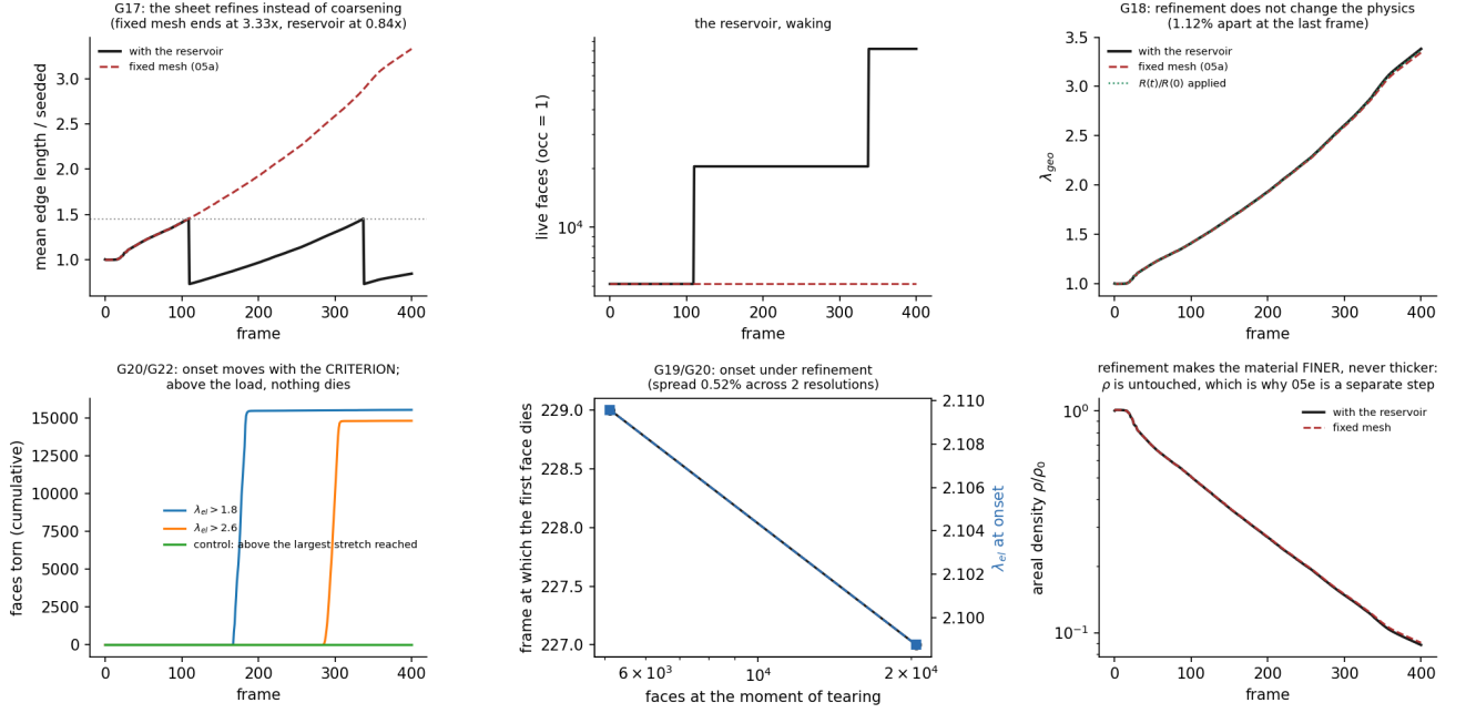
Figure 7: 05d_tear: tearing, and the gate the MPM sheet was never given. Bottom middle G19 : the same criterion at 5,115 and 20,471 faces tears at \lambda^{\text{el}} = 2.110 and 2.099 — 0.52% apart, against a 5% threshold — so the tear is set by the material and not by the discretisation. Bottom left G20, G22 : onset moves with the criterion (frames 167 / 227 / 285 at thresholds 1.8 / 2.2 / 2.6) and a criterion above the largest stretch reached kills 0 of 81,920 faces — which is the run-127 control, run on purpose. Top row G17, G18 : the reservoir holds the edge length at 0.84 of seeded where a fixed mesh reaches 3.33, and refinement improves the fidelity rather than merely preserving it.
