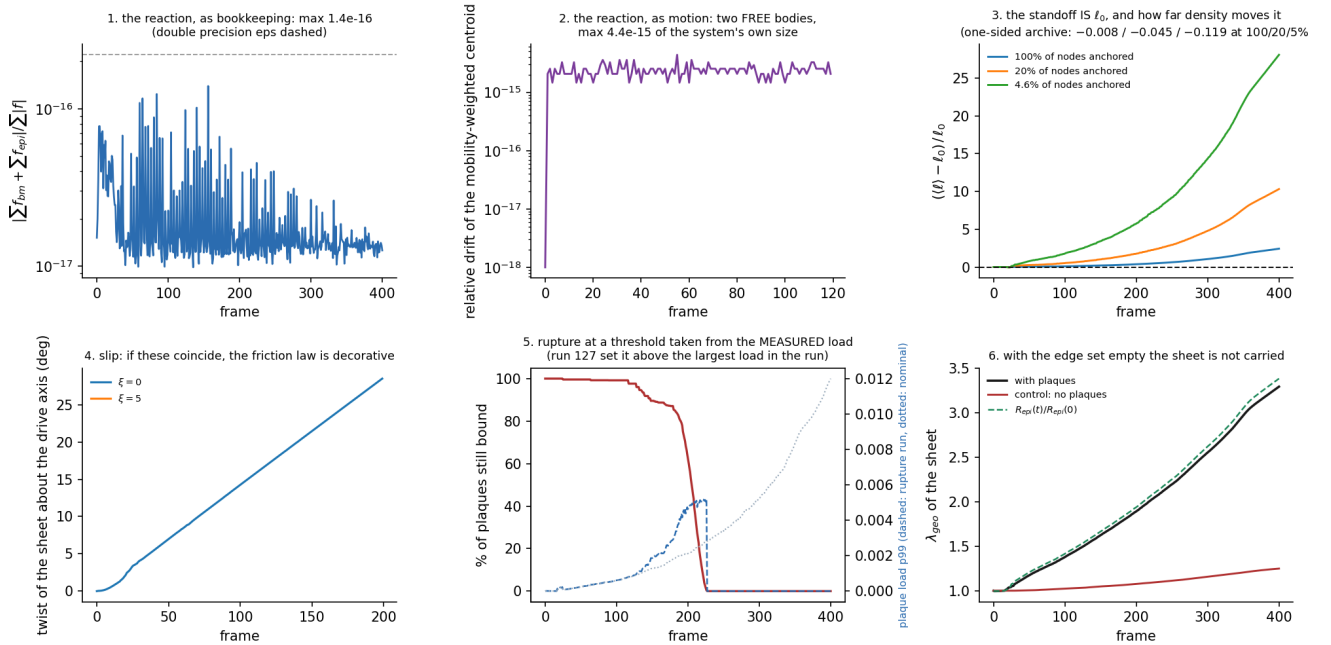
Figure 4: 05b_plaque, the adhesion as an edge set. 1 G9 : the residual on the adhesion's own force pair sits at 1.4 \times 10^{-16} , i.e. at double-precision \varepsilon — one operator, a delta to both endpoints, and the reaction cannot be half-implemented. 2 G10 : the same claim as motion, with two free bodies whose mobility-weighted centroid drifts by 4.4 \times 10^{-15} of the system's own size. 3 G12 : the standoff is 3.43 \ell_0 and not \ell_0 . 4 G13 : \xi = 0 and \xi > 0 do not separate, because a fixed barycentric anchor is a tangential pin. 5 rupture is a clock rather than a load, for want of turnover. §4.2 is what each of those three costs, and §2.3 is the scheme that replaces them.
