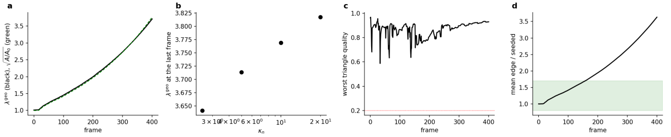
Figure 3: 05q_gates : G40–G46 on the real epithelium, 05b's rig with the driver swapped and nothing else changed. a G41 : \lambda^{\text{geo}} (black) on the apical-area ratio \sqrt{A_{\text{ep}}(t)/A_{\text{ep}}(0)} (green) to 1.40% over 401 frames — the sheet is reporting the tissue's growth, and against the area , since a dividing epithelium is not a sphere and the radius ratio would have been the wrong reference. b G40 at 4.72% over 8\times in \kappa_n , and the four points are monotone: passed, but the adhesion's compliance is in there. c G42 : worst triangle quality 0.587, far above the 0.2 line, against 0.000 for the vertex-plaque driver this replaces. d G44 : with no bm_refine the mean edge reaches 3.63\times its seeded length, outside the band (green) — the failure is expected and its value is the measurement, i.e. how much refinement a 3.77\times dilation of a real surface demands.
