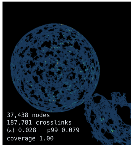
no adhesion k_{\text{adh}} = 0
