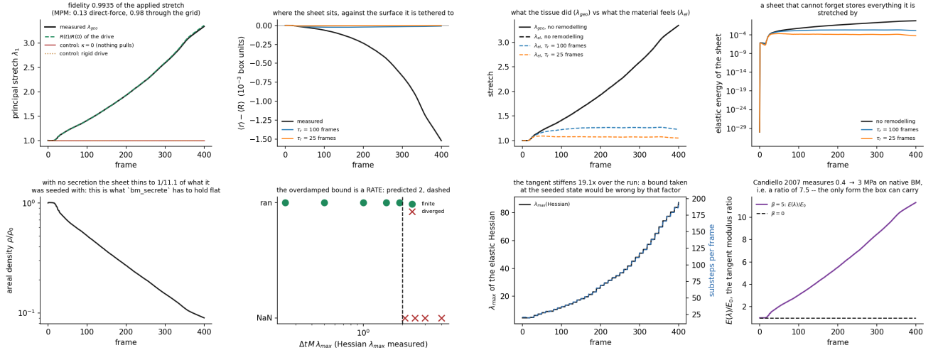
Figure 3: 05a_sheet, the sheet alone on the recorded epithelial surface. a G5 : the measured \lambda^{geo} lies on the applied R(t)/R(0) to 0.9935, against 0.13 for the MPM sheet moved by an engine delta; the two flat lines at 1.0000 are G6 ( \kappa = 0 ) and G7 (a rigid drive), i.e. the measure invents no strain and does not mistake motion for deformation. b-c remodelling: at \tau_r = 25 frames the standoff improves 1026 \times while \lambda^{geo} is unmoved — the sheet still goes where the tissue puts it and stops fighting. f G8 : divergence at the predicted group \Delta t M \lambda_{max} = 2 , measured, not assumed. g the tangent stiffens 19 \times over the run, which is why the bound has to be re-measured. h the stiffening law as a ratio, since MPa is not a quantity this box has.
