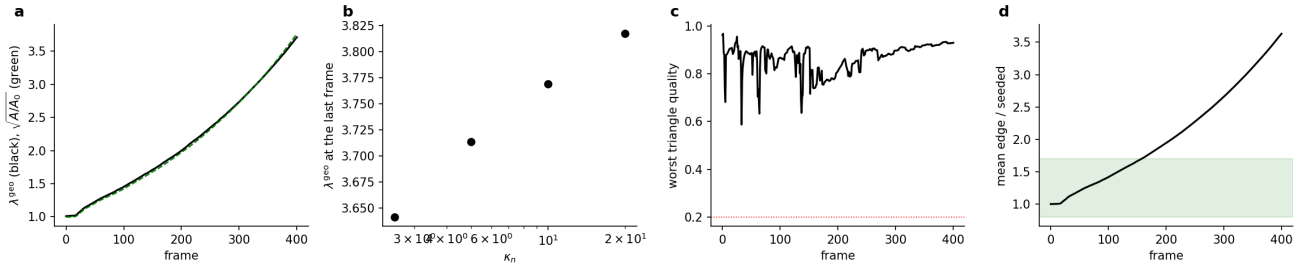
Figure 3: 05k_gates : G40–G46 on the real epithelium, 05b's rig with the driver swapped and nothing else changed. a G41: \lambda^{\text{geo}} (black) on the apical-area ratio \sqrt{A_{\text{ep}}(t)/A_{\text{ep}}(0)} (green) to 1.40% over 401 frames — the sheet is reporting the tissue's growth, and against the area , since a dividing epithelium is not a sphere and the radius ratio would have been the wrong reference. b G40 at 4.72% over 8\times in \kappa_n , and the four points are monotone: passed, but the adhesion's compliance is in there. c G42: worst triangle quality 0.587, far above the 0.2 line, against 0.000 for the vertex-plaque driver this replaces. d G44: with no bm_refine the mean edge reaches 3.63\times its seeded length, outside the band (green) — the failure is expected and its value is the measurement, i.e. how much refinement a 3.77\times dilation of a real surface demands.
