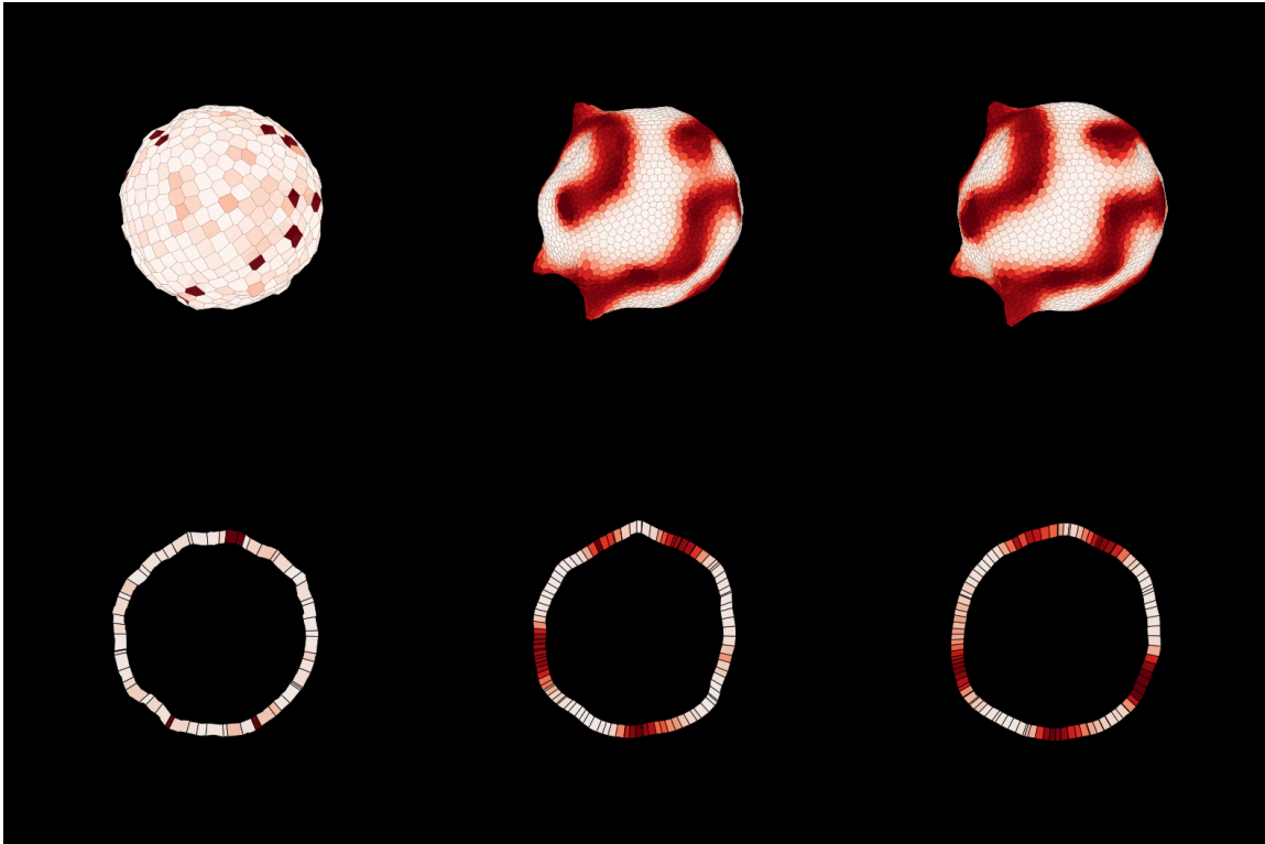
Figure 3: Divide-on-activation ( ext4_tight ): cells divide directly where the activator exceeds a threshold, no growth. The most pattern-faithful extrusion ( \text{corr}(a, r) = 0.29 ) — the lobes and protrusions sit on the activator (dark) bands, on a clean single-sheet monolayer (cross-section, bottom).
