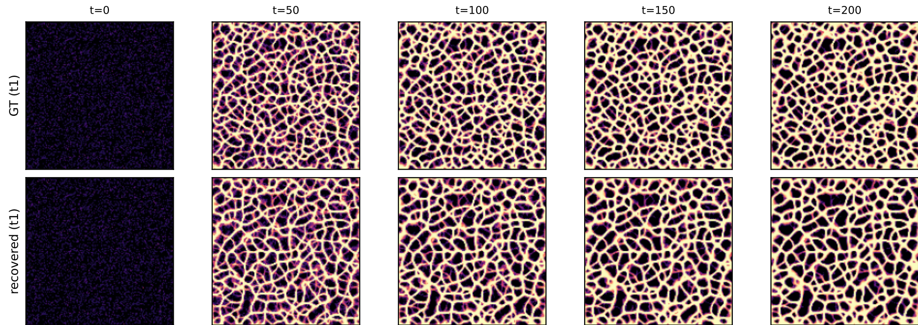
Target 1 -- chemical field: GT vs position-loss recovery
