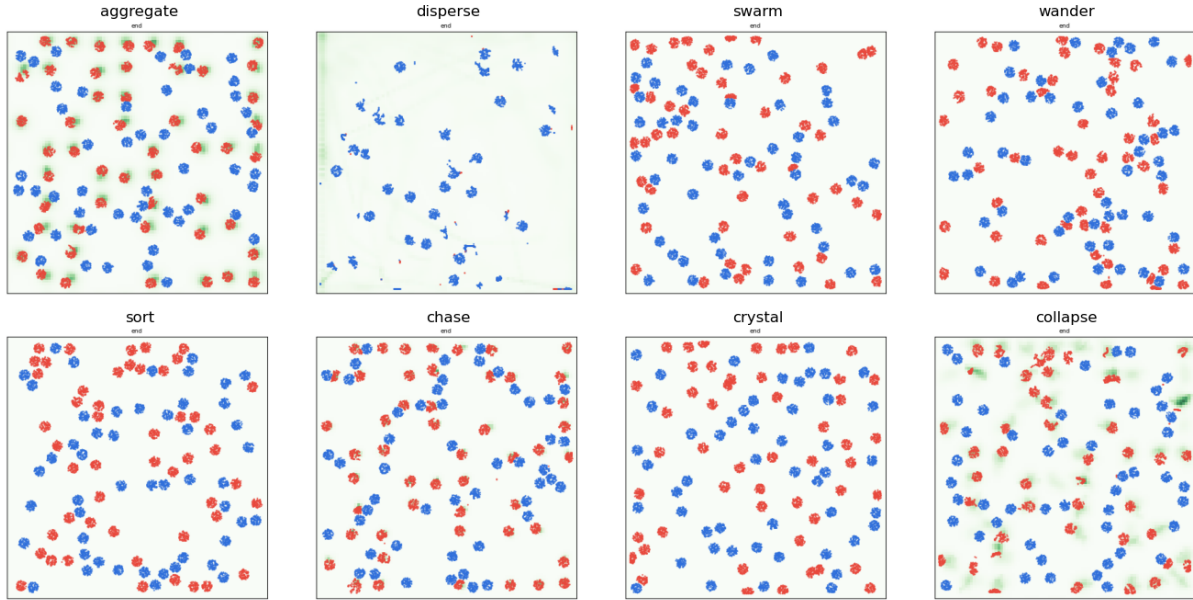
Figure 3: End states of the eight simulations described above, all generated from the same operator registry by changing only the spec.
