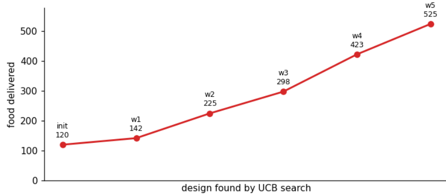
Figure 7: Optimizing the colony. Best food delivered as UCB searches the eight-parameter design space, from the initial hand-set design to the best found — a slow, soft, high-drag, many-celled colony.
