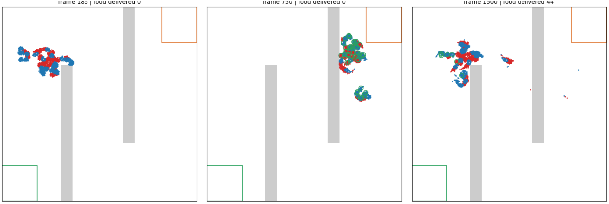
Figure 6: Maze foraging. Two rigid populations (red, blue) leave home (green box, bottom-left), thread the walls (grey) up the food gradient to the source (orange box, top-right), pick up food (green ring), and return home along the home gradient to drop it off. The delivered count rises as the colony forages.
