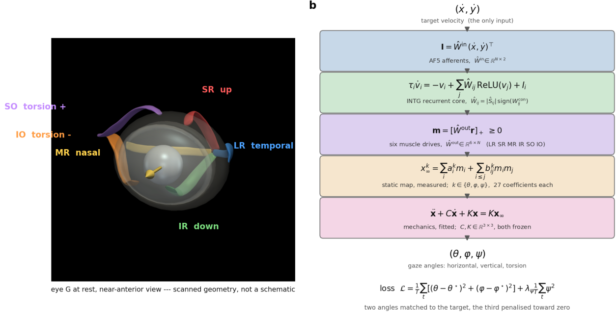
Figure 3: The eye, and the symbols of the model. (a) The globe seen down the corneal axis with the six extraocular muscles at their true insertions, drawn from eye_anatomy.MUSCLES — the same table the MPM uses to shape the straps, so this is the model's own geometry. Only the horizontal pair is innervated by this circuit: LR abducts (positive gaze), MR adducts. The four faint muscles exist in the eye but receive no command. The two axes the model uses are marked: horizontal gaze \theta , positive in abduction, and vertical gaze \varphi . (b) Every symbol of the nine steps below, in the order the signal meets them: the target velocity (\dot{x}, \dot{y}) , the input map \hat{W}^{\text{in}} onto the AF5 afferents, the sign-locked recurrent core, the output map \hat{W}^{\text{out}} onto four non-negative motor pools, the push-pull commands u_{\theta}, u_{\varphi} , the frozen per-axis eye, and the loss on the gaze angles (\theta, \varphi) — after the eye, not on the command. Regenerate with python fit_plant.py and python fig_eye_schematic.py in Plexus/prototype/eye .
