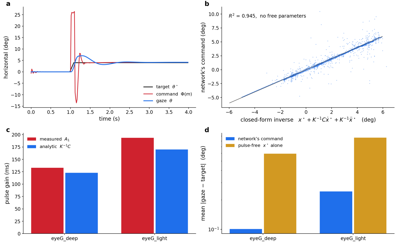
Figure 5: The controller learned the eye’s inverse, not a tracking habit. (a) A step probe: the target steps 4^\circ and holds. The corpus contains no steps — it is splines at three speeds — so this regime is new to the network. The command goes to +26, brakes to -14, then settles on the +4 step, while the gaze rises smoothly to the target: accelerate, brake, hold. The doublet is the K^{-1}\ddot{x}^* term and the offset that survives it is x^* . (b) The network’s command against the closed-form inverse above, evaluated with the eye’s own K and C and no free parameters : R^2 = 0.945 . Fitting A_0, A_1, A_2 freely reaches only 0.952, so the analytic matrices cost essentially nothing. (c) The velocity gain A_1 of each network against its own K^{-1}C . The two eyes differ by 46 % in measured pulse gain (133 against 193 ms) and each matches its own plant; a pulse that was a habit of the architecture or of the corpus would be the same in both. (d) Necessity: drive each eye with the pulse-free command x^* and the tracking error rises 5.9\times on the deep eye ( 0.101 \rightarrow 0.592^\circ ) and 3.5\times on the light one. Regenerate with python fig_pulse_step.py in prototype/dot_tracking .
