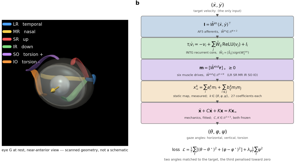
Figure 3: The eye, and the symbols of the model. (a) Eye G at rest, near-anterior view, drawn by the surface renderer from the scanned geometry rather than schematised: the translucent globe, the lens, and the six straps as the Blender reconstruction places them. Muscle actions in the legend are the ones stage 0 measured, not the textbook ones — SO elevates and torts positive here, IO depresses, because both obliques pull from the rostral orbit with no trochlea to reverse the superior one. Only the horizontal pair is innervated by this circuit: LR abducts (positive gaze), MR adducts. The four faint muscles exist in the eye but receive no command. The two axes the model uses are marked: horizontal gaze \theta , positive in abduction, and vertical gaze \varphi . (b) Every symbol of the nine steps below, in the order the signal meets them: the target velocity (\dot{x}, \dot{y}) , the input map \hat{\mathbf{W}}^{\text{in}} onto the AF5 afferents, the sign-locked recurrent core, the output map \hat{\mathbf{W}}^{\text{out}} onto four non-negative motor pools, the push-pull commands u_{\theta}, u_{\varphi} , the frozen per-axis eye, and the loss on the gaze angles (\theta, \varphi) — after the eye, not on the command. Regenerate with python fit_plant.py and python fig_eye_schematic.py in Plexus/prototype/eye .
