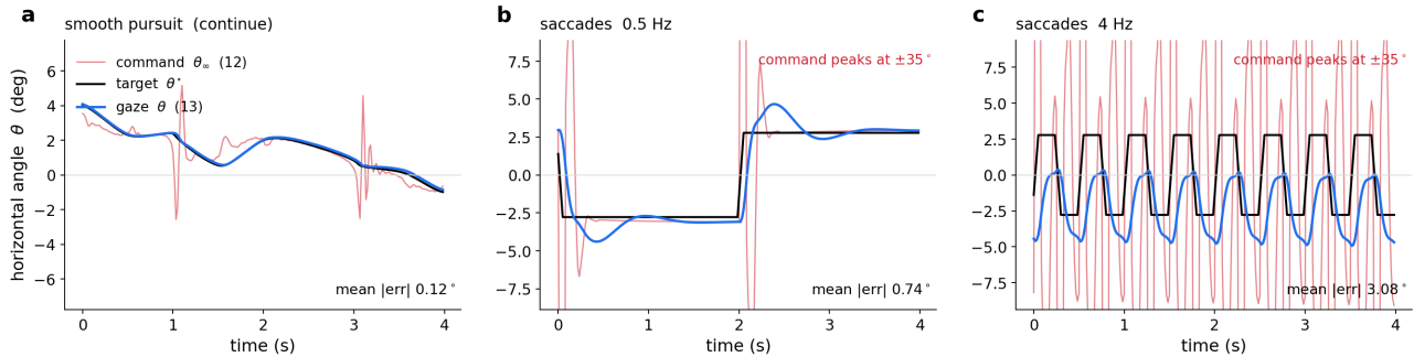
Figure 5: The six-drive controller on eye G, three regimes. Horizontal angle only, four seconds of each, drawn from the same rollout the movies play. Black is the target \theta^* , blue the gaze \theta of (13), red the command \theta_\infty of (12) — the angle the eye would settle at if the drives froze. (a) Smooth pursuit: blue sits on black, and red departs from both only at the direction reversals, where the pulse of section 5.2 is needed. (b) Saccades at 0.5 Hz: the gaze reaches each new angle in about a third of a second and overshoots slightly, and the command is a doublet reaching \pm 35^\circ — an order of magnitude beyond the \pm 2.8^\circ excursion, which is why the axis is scaled to the target and the gaze and the command leaves the panel. (c) Saccades at 4 Hz, where the half-period of 125 ms is the eye’s own group delay of 127 ms: the gaze is still travelling toward one target when the next arrives, so it never reaches either and tracking has stopped in any useful sense. Regenerate with python fig_eyeG_traces.py in prototype/dot_tracking .
