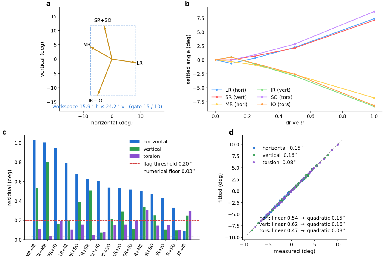
Eye G, characterised. (a) Stage 0-lite: the four cardinal synergies driven open loop, each arrow the settled gaze excursion, the dashed box the workspace they span — 15.9^\circ horizontal by 24.2^\circ vertical, against the 15/10 the task needs. All four move the eye in the direction the insertions predict, which is what says the scanned anatomy is right. (b) Stage 1: the six marginals on each muscle’s own dominant axis. The plant is nearly dead below u \approx 0.25 and does most of its work in the upper half of the drive range, so a linearisation about rest is wrong in the direction that matters. (c) Stage 2a: the residual of each pair against its additive prediction, per angle, with the flag threshold and the numerical floor. All fifteen pairs interact, mostly in horizontal. (d) Stage 6d: the quadratic g of (4) fitted over 64 Sobol points in [0, 1]^6 , measured against fitted. Regenerate with python Plexus/prototype/eye/fig_eyeG_charac.py .
