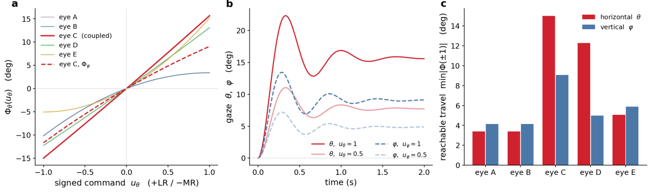
The identified eye models. All three panels are drawn from the stored fit in plant.npz / plant_v.npz , in the symbols of section 5. (a) The static nonlinearity \Phi_\theta(u_\theta) of all five eyes, and \Phi_\phi of eye C, the one the controller is coupled to. Every curve is monotone by construction; the curvature is the genuine asymmetry between abduction and adduction. (b) Step response of eye C on both axes at commands 0.5 and 1: the overshoot and the ringing are what only the inertial term can produce, and they are the reason the second-order eye beats the first. (c) Reachable travel per axis, \min|\Phi(\pm 1)| — the quantity that decides whether a tracking task is expressible at all, and the reason the world is scaled anisotropically. Regenerate with python fig_plant_summary.py in Plexus/prototype/eye .
