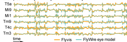
d Examples FlyWire eye model vs Flyvis rollouts
