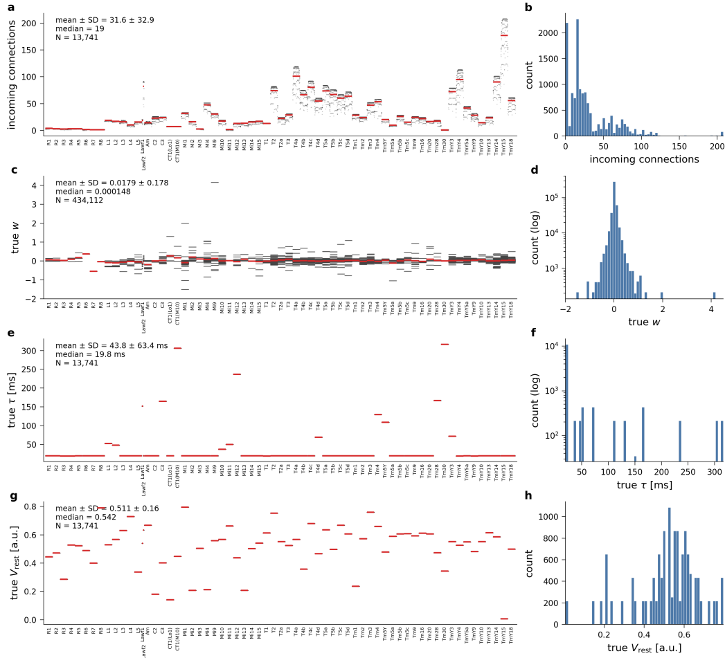
Supplementary Figure 6: Ground-truth circuit-parameter distributions of the central 217-column Flyvis model (13,741 neurons, 65 cell types, 434,112 synaptic edges). (a) Number of incoming synaptic connections per neuron (one dot per neuron, sorted by cell type; red horizontal lines mark the per-type mean). (b) Marginal histogram of the same quantity. (c) True synaptic weight W_{ij} , one dot per edge ( y = w_{j \rightarrow i} plotted at x = i ). (d) Per-edge weight histogram (log y ); sharply peaked at 0 with a thin tail to w \approx 4 . (e) True membrane time constant \tau_i . (f) \tau histogram (log y ); bimodal with \sim 79\% of neurons at \tau \approx 25 ms and a sparse tail out to \sim 320 ms. (g) True resting potential V_i^{\text{rest}} . (h) V^{\text{rest}} histogram; concentrated in 0.4–0.7. Top-left of each left-column panel: mean, median, and sample size.
