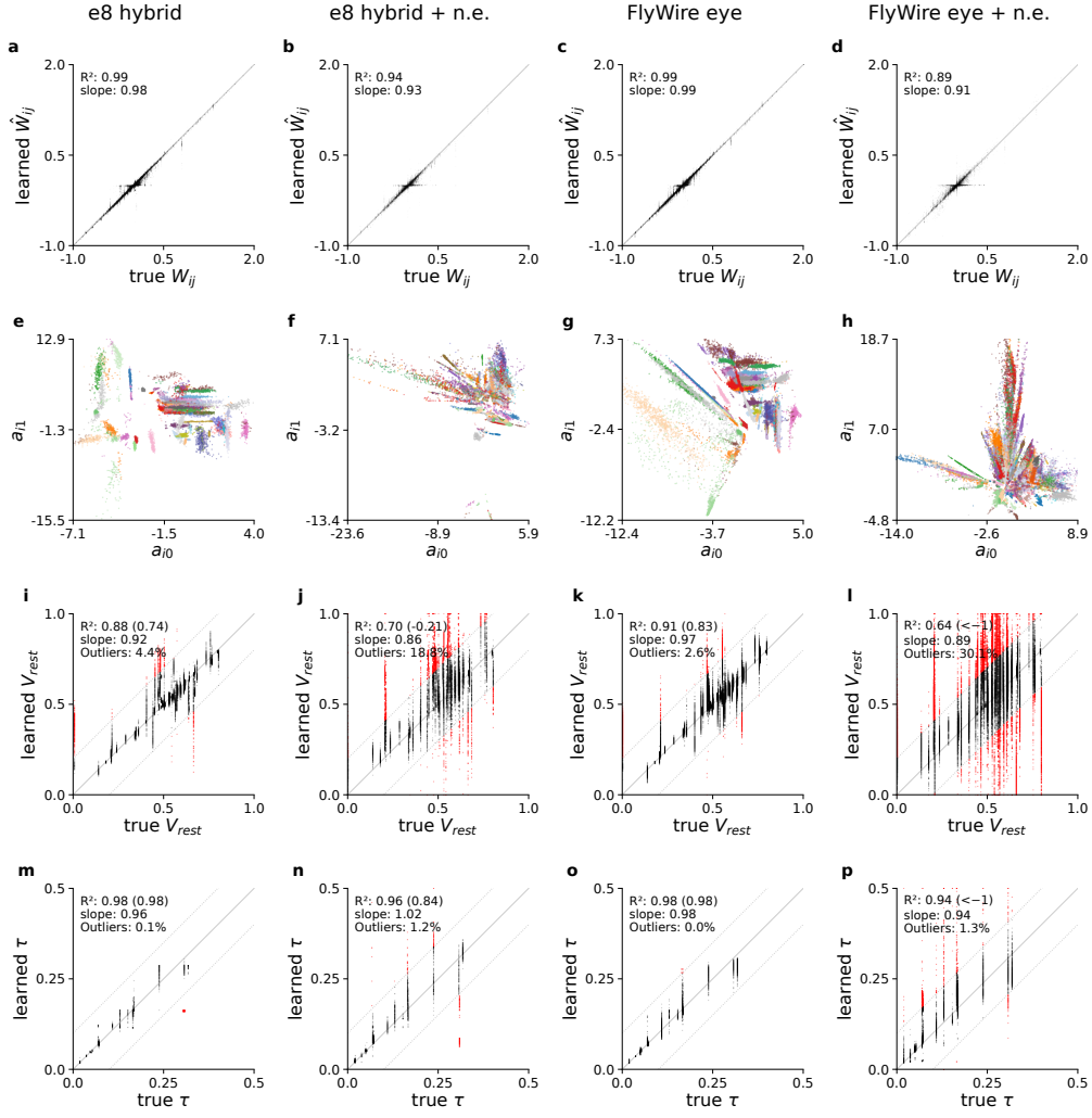
Supplementary Figure 11: Circuit parameter extraction from the general-form GNN (group lasso 25) on the four FlyWire connectome variants with low model noise ( \sigma = 0.05 ; fold cv00 of experiment 7): e8 hybrid, e8 hybrid with proximal null edges (n.e.), FlyWire eye, and FlyWire eye with proximal null edges. (a–d) Learned against true synaptic weight \hat{W}_{ij} over the edges fitted by the template readout (60%, 61%, 59% and 62% of the edges). (e–h) Learned latent embeddings \mathbf{a}_i \in \mathbb{R}^2 of all neurons, coloured by ground-truth cell type. (i–l) Resting potentials V_i^{rest} and (m–p) time constants \tau_i of the template readout, outliers beyond the dotted \pm 0.2 / \pm 0.1 s bands in red; R^2 (inlier, all-neuron in parentheses), slope and outlier fraction as in Tab. 2.
