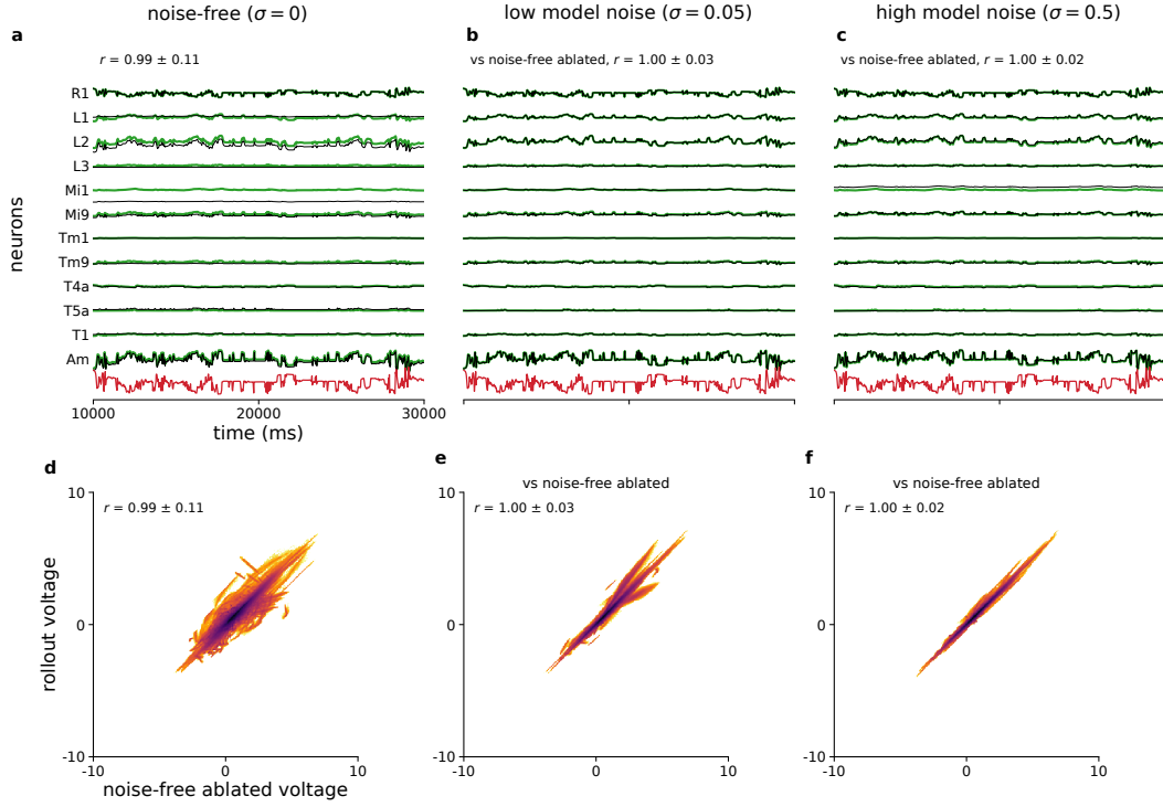
Supplementary Figure 9: Rollout prediction under 50% edge ablation. General-form GNN (group lasso 25; fold cv00 of experiment 2) evaluated on central 217-column Flyvis data under three model noise regimes (noise-free \sigma = 0 , \sigma = 0.05 , \sigma = 0.5 ), tested on held-out stimuli, and compared against the noise-free ablated Flyvis simulation. For each test the simulator regenerates voltage traces with 50% of the synaptic edges zeroed, and the same edge mask is applied to the trained GNN's learned weights \hat{\mathbf{W}} before rollout (no retraining). Top row ( a , b , c ): GNN rollout traces for 12 representative cell types over a 20 s window (1,000 frames at \Delta t = 20 ms). Green: ablated ground-truth voltage; black: GNN rollout prediction; red: the visual input of the photoreceptor row. Bottom row ( d , e , f ): rollout voltage against the noise-free ablated voltage, pooled over all (neuron, frame) pairs of the 7,999-frame rollout as a log-density image. Pearson r : per-neuron, Fisher- z pooled, on the full rollout.
