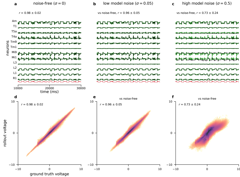
Supplementary Figure 21: EED model rollout prediction: EED model evaluated on central 217-column Flyvis data under three model noise regimes ( \sigma = 0 , \sigma = 0.05 , \sigma = 0.5 ), tested on held-out stimuli, and compared against noise-free Flyvis simulations. Top row (a, b, c): rollout traces for 12 representative cell types over a 20 s window (1,000 frames at \Delta t = 20 ms). Green: ground-truth voltage; black: Recurrent MLP rollout prediction; red: one visual input stimulus. Bottom row (d, e, f): scatterplots of rollout voltage vs noise-free ground-truth voltage, pooled over all (neuron, frame) pairs and subsampled to 2 \cdot 10^6 points for display. Pearson r computed on the full 8,000-frame rollout. Note the degradation in performance with the addition of model noise across columns.
