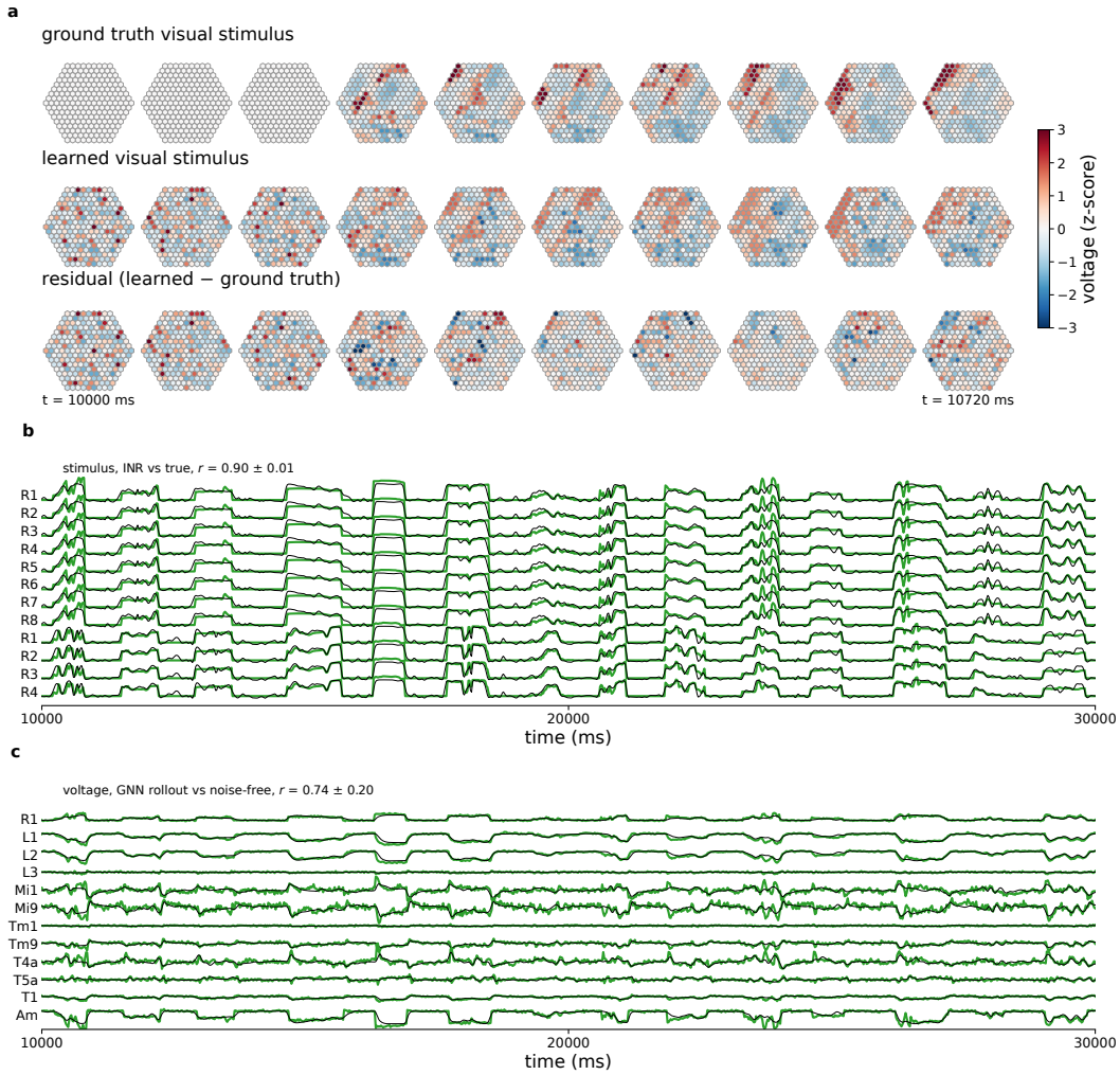
Supplementary Figure 10: Joint GNN+INR (visual SIREN): the general-form GNN (group lasso 25, one-step training) evaluated on central 217-column Flyvis data with low model noise ( \sigma = 0.05 ), 64 000 training frames (fold cv00 of experiment 11); rollout evaluated on the first 7,999 training frames since the SIREN cannot extrapolate to test-time indices. The SIREN output is shown with its mean and SD matched to the true stimulus, sign from the correlation (its raw output is defined up to the sign and scale the GNN’s input weights absorb; the tester’s least-squares correction would compress the learned range by the factor r ). (a) INR-reconstructed visual stimulus on the R1 photoreceptor lattice (217 columns), ten frames spaced by 80 ms from 10,000 ms, z -scored per frame; top: ground truth; middle: INR; bottom: residual. (b) INR stimulus (black) against the true one (green) for 12 photoreceptors (R1–R8 of one column, R1–R4 of another) over a 20 s window (1,000 frames at \Delta t = 20 ms); the header gives the per-photoreceptor Pearson r over the 7,999 frames, Fisher- z pooled over the 1,736 photoreceptors (mean \pm SD). The SIREN’s output enters the GNN squared, so it cannot be negative, and f_\theta is free to read it with either sign; this run learned the inverted code (bright pixels \rightarrow small output), so its zero floor becomes a ceiling at 0.73 of the true range: the 7% of photoreceptor–frames brighter than it all receive the same input, visible as the flattened bright plateaus. The sign is set at random by the training (4 of the 5 folds learned it inverted). (c) GNN voltage rollout (black) against the noise-free ground truth (green) for 12 representative cell types over the same window; the header gives the per-neuron Pearson r , Fisher- z pooled over all 13,741 neurons (mean \pm SD).
