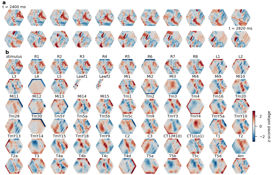
Supplementary Figure 4: Visual input and per-cell-type activity on the retinotopic hexagonal lattice (central 217-column Flyvis model, noise-free, 13,741 neurons, 1,736 photoreceptors, 434,112 synaptic connections, integration step \Delta t = 20 ms). (a) Consecutive frames of the visual stimulus ( t = 2400 – 2820 ms, one panel every 20 ms) projected on the hex lattice of photoreceptors. Each frame is z-scored across photoreceptors so that local contrast pattern is visible. (b) Snapshot of the voltage at t = 2400 ms for the stimulus (top-left) and the 65 cell types. Values are z-scored within each cell type, so every hexagon panel shares the same color scale (shown on the right). Red (positive) and blue (negative) indicate deviations from the type's mean voltage at that instant; white is at the mean.
