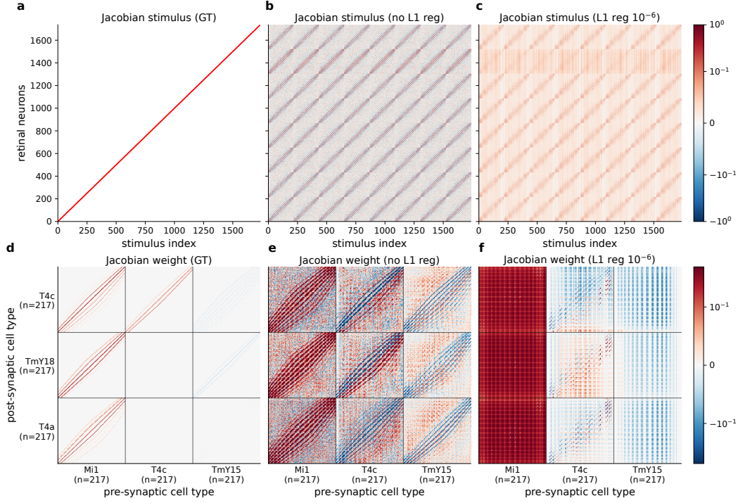
Supplementary Figure 19: Jacobian of Recurrent MLP does not capture the true dynamics We compute the Jacobian of the right hand side of Supp. Eq. 20 with respect to the input stimulus (top row) and the past neural activity (bottom row). For the sake of display we restrict the view to specific entries of the Jacobian that help visually distinguish the learned dynamics from the true simulation update in Eq. (1). In the top row a-c we show the Jacobian of the 1736 retinal neurons with respect to the 1736 input stimuli. a shows the ground truth, where stimulus i is fed into retinal neuron i with unit strength. b shows the Jacobian of the learned MLP update, which displays an interesting structure with a periodic motif repeating every 217 indices mirroring the columnar arrangement. This shows that the MLP learned a different assignment between the 1736 stimuli and the 13,741 neurons that nevertheless captures the one-step and rollout properties of the true dynamics accurately. c shows the impact of L1 regularization that is added to force sparsity of learned dynamics. While the true solution is also sparse, the broad L1 penalty finds a completely different sparse solution to the problem. The bottom row d-f shows the Jacobian with respect to the past neural activity, where we have restricted the view to three pre and post-synaptic cell types. a shows the ground truth weights from the Flyvis model, b shows the result from the MLP model without regularization and c shows the result with the addition of regularization. Again we see the same pattern as with the stimulus. Color bars in all figures use a symmetric-log normalization (linthresh = 0.1) so small magnitudes remain visible; each row shares one colorbar.
