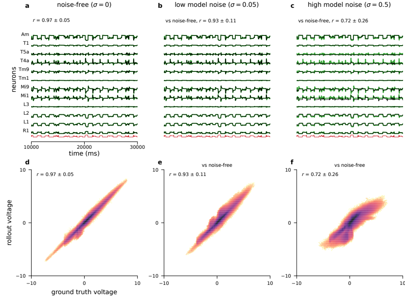
Supplementary Figure 18: Recurrent MLP rollout prediction: Recurrent MLP evaluated on central 217-column Flyvis data under three model noise regimes ( \sigma = 0 , \sigma = 0.05 , \sigma = 0.5 ), tested on held-out stimuli, and compared against noise-free Flyvis simulations. Top row ( a , b , c ): rollout traces for 12 representative cell types over a 20 s window (1,000 frames at \Delta t = 20 ms). Green: ground-truth voltage; black: Recurrent MLP rollout prediction; red: one visual input stimulus. Bottom row ( d , e , f ): scatterplots of rollout voltage vs noise-free ground-truth voltage, pooled over all (neuron, frame) pairs and subsampled to 2 \cdot 10^6 points for display. Pearson r computed on the full 8,000-frame rollout. Note the degradation in performance with the addition of model noise across columns.
