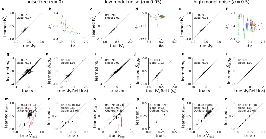
Figure 1: Circuit parameter extraction from the general-form GNN ( g_\phi = \text{MLP}(\mathbf{a}_i, \mathbf{a}_j, v_i, v_j) , group lasso 25) on Flyvis-217 under three model-noise regimes ( \sigma = 0, 0.05, 0.5 ; fold cv00 of experiment 2). (a, c, e) Learned against true synaptic weight \hat{W}_{ij} , one point per edge fitted by the template readout (77%, 76% and 96% of the 434,112 edges at \sigma = 0, 0.05, 0.5 ; the rest have a presynaptic neuron that never rises above the activity floor). (b, d, f) Learned latent embeddings \mathbf{a}_i \in \mathbb{R}^2 of all neurons, coloured by ground-truth cell type. (g, i, k) The aggregated message m_i = \sum_j \hat{W}_{ij} g_\phi(\cdot) each neuron receives, learned against the generator’s \sum_j W_{ij} \text{ReLU}(v_j) , on the frames the metric R_m^2 is scored on (the general-form circuit counterpart of the published f_\theta panel). (h, j, l) The per-edge message at observed (v_i, v_j) : learned k_i \hat{W}_{ij} g_\phi(\mathbf{a}_i, \mathbf{a}_j, v_i, v_j) against the generator’s W_{ij} \text{ReLU}(v_j) on 1,024 random edges \times 64 random frames, k_i the template readout’s per-neuron gauge (the counterpart of the published g_\phi panel). (m, o, q) Resting potentials V_i^{\text{rest}} . (n, p, r) Time constants \tau_i . Each scatter is annotated with the R^2 and slope of learned against true quoted in Tab. 1 (identity-line R^2 ; for \tau and V^{\text{rest}} the inlier R^2 with the all-neuron R^2 in parentheses, outliers beyond the dotted \pm 0.1 s / \pm 0.2 bands in red and their fraction printed); the per-neuron \tau , V^{\text{rest}} and per-edge \hat{W}_{ij} are the template readout’s (Appendix F.2).
