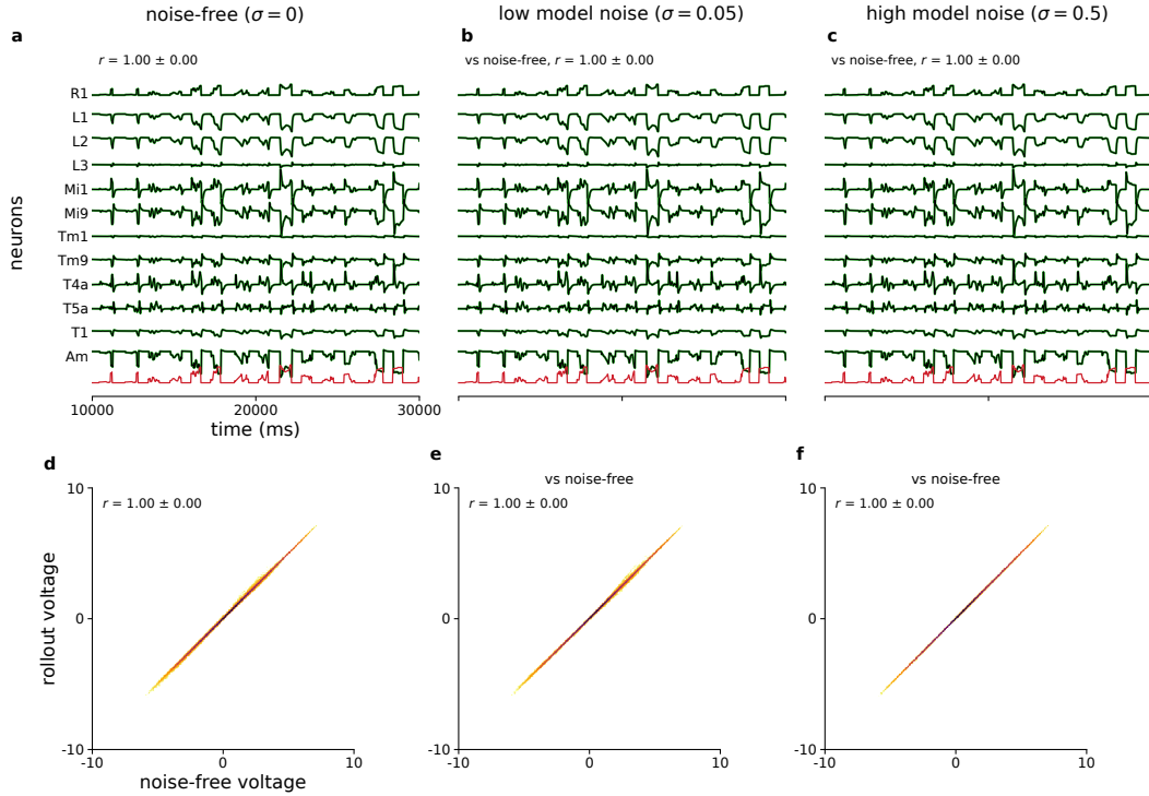
Supplementary Figure 15: Known-ODE rollout prediction. Known-ODE models (the published checkpoints, fold cv00, re-analysed with the current analysis code, experiment 15) evaluated on central 217-column Flyvis data under three model noise regimes ( \sigma = 0 , \sigma = 0.05 , \sigma = 0.5 ), tested on held-out stimuli, and compared against the noise-free Flyvis simulation of the same stimuli. Top row (a, b, c): Known-ODE rollout traces for 12 representative cell types over a 20 s window (1,000 frames at \Delta t = 20 ms). Green: noise-free ground-truth voltage; black: Known-ODE rollout prediction; red: the visual input of the photoreceptor row. Bottom row (d, e, f): rollout voltage against noise-free ground-truth voltage, pooled over all (neuron, frame) pairs of the 7,207-frame rollout as a log-density image. Pearson r : per-neuron, Fisher- z pooled, on the full rollout.
