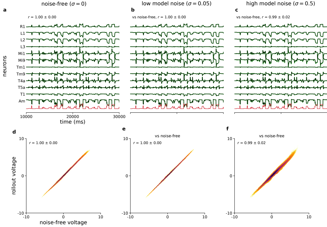
Supplementary Figure 7: Rollout prediction. General-form GNN (group lasso 25) evaluated on central 217-column Flyvis data under three model noise regimes ( \sigma = 0 , \sigma = 0.05 , \sigma = 0.5 ; fold cv00 of experiment 2), tested on held-out stimuli, and compared against the noise-free Flyvis simulation of the same stimuli. Top row ( a , b , c ): GNN rollout traces for 12 representative cell types over a 20 s window (1,000 frames at \Delta t = 20 ms). Green: noise-free ground-truth voltage; black: GNN rollout prediction; red: the visual input of the photoreceptor row. Bottom row ( d , e , f ): rollout voltage against noise-free ground-truth voltage, pooled over all (neuron, frame) pairs of the 7,207-frame rollout (the fold's held-out stimuli) as a log-density image. Pearson r : per-neuron, Fisher- z pooled, on the full rollout.
