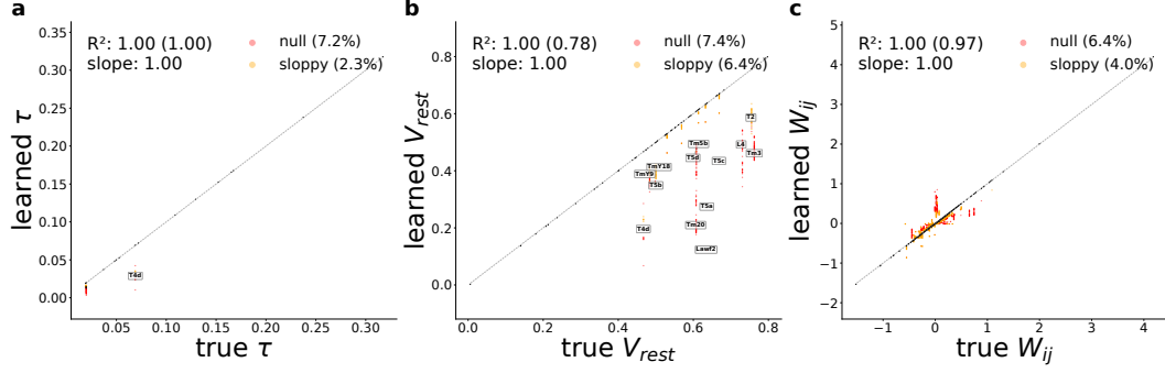
Supplementary Figure 13: Per-neuron least-squares recovery of the ground-truth ODE parameters on noise-free Flyvis data. Each panel scatters the recovered value against the ground truth; the dashed line is y = x . (A) membrane time constant \tau_i ; (B) resting voltage V_i^{\text{rest}} ; (C) synaptic weight W_{ij} . Black points are well-identified; orange (“sloppy”) and red (“null”) points lie in poorly-conditioned directions of the per-neuron Gram matrix and are flagged as degenerate by the eigendecomposition. We report R^2 over the well-identified subset (with the all-points R^2 in parentheses) and the regression slope on the same subset. Fractions in the legend indicate the fraction of parameter dimensions that have non-zero inner product with a null or sloppy direction; in panels A, B it is the fraction of neurons, and in panel C it is the fraction of edges.
