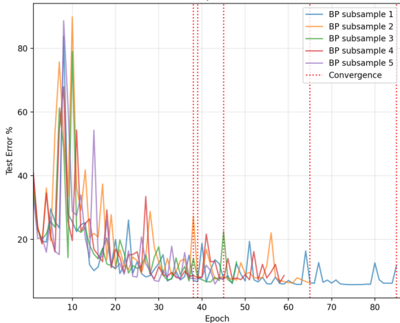
BP - Sample Size 5000
