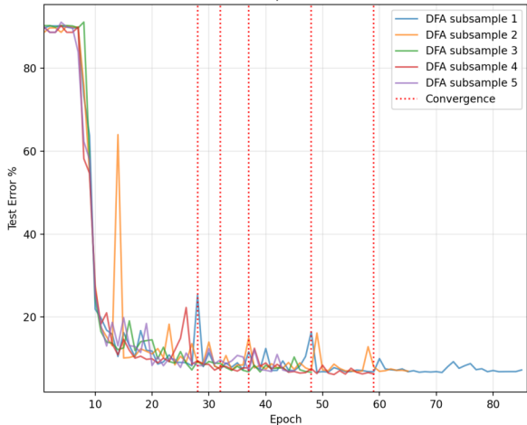
DFA - Sample Size 5000
