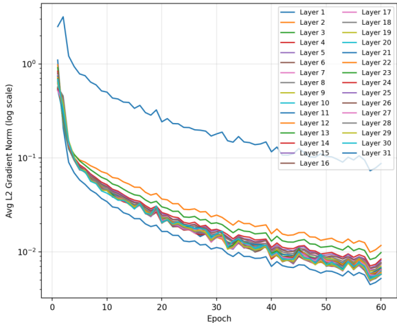
DFA Gradient Norms
