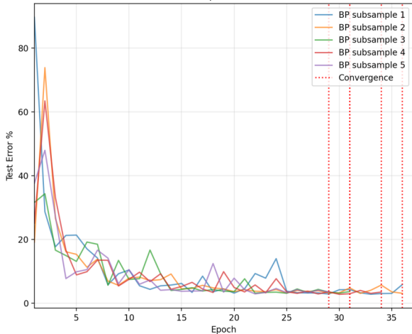
BP - Sample Size 30000
