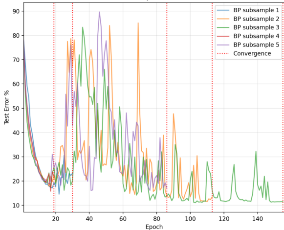
BP - Sample Size 1000
