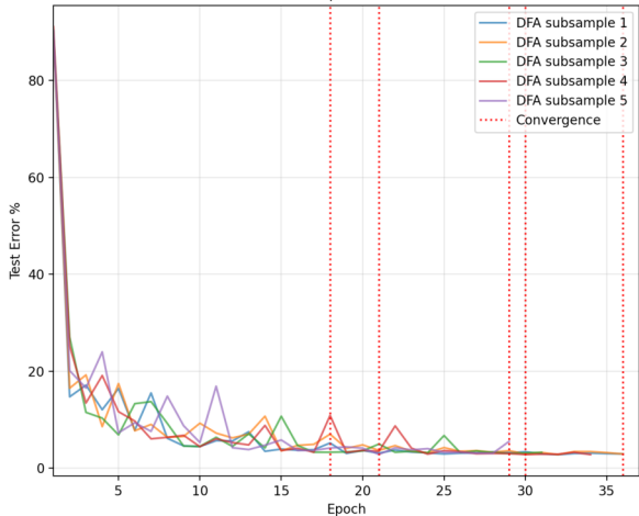
DFA - Sample Size 30000
