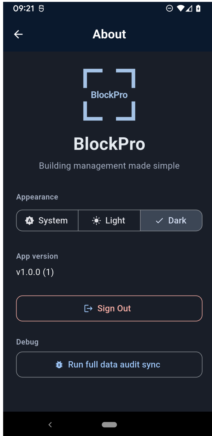
About — dark
