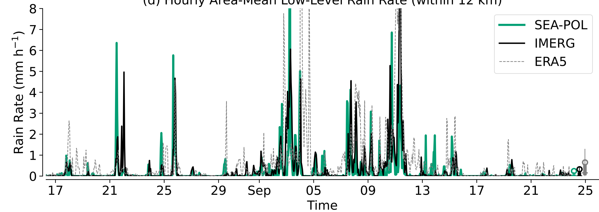
(d) Hourly Area-Mean Low-Level Rain Rate (within 12 km)
