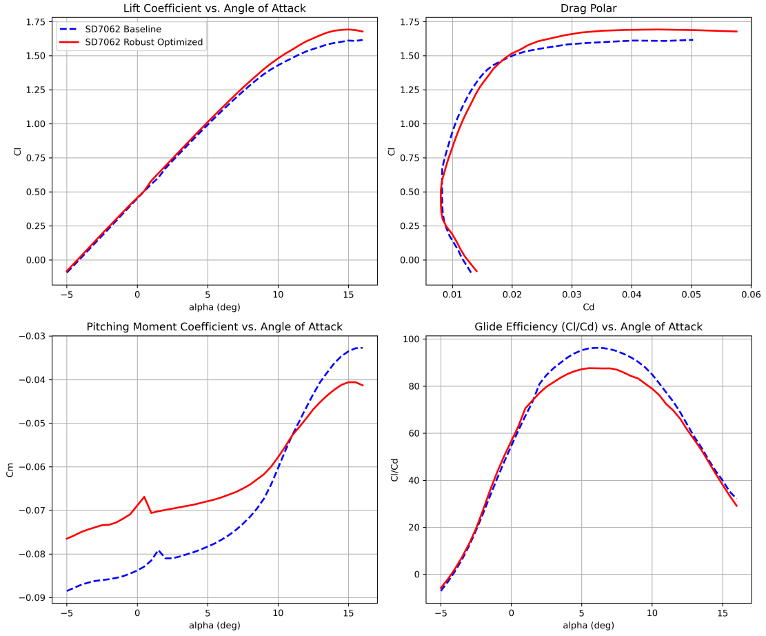
Figure 3: Aerodynamic Performance Comparison: Lift Curve ( C_L vs \alpha ), Drag Polar ( C_L vs C_D ), Moment Curve ( C_m vs \alpha ), and Glide Efficiency ( C_L/C_D vs \alpha ).
