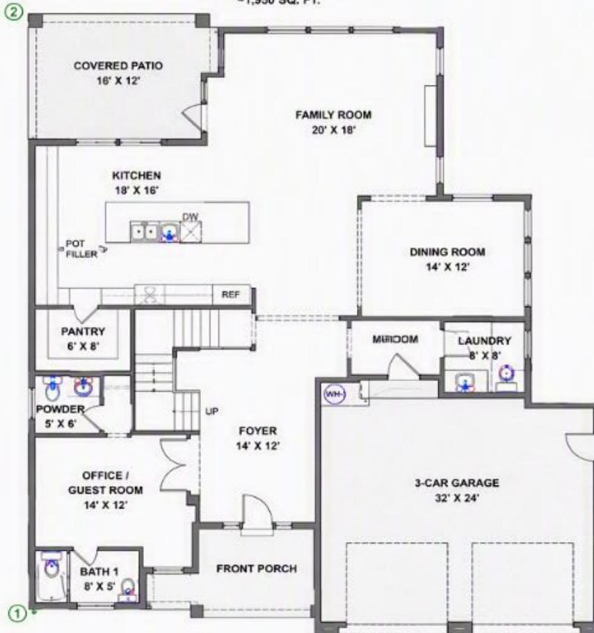
FIRST FLOOR PLAN ~1,950 SQ. FT.
