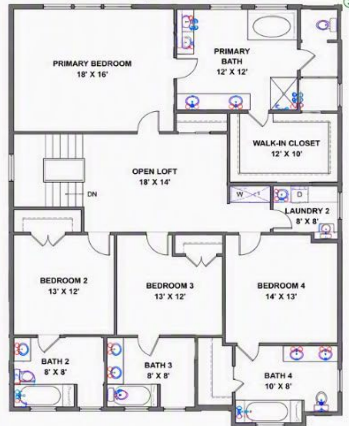
SECOND FLOOR PLAN ~1,700 SQ. FT.
