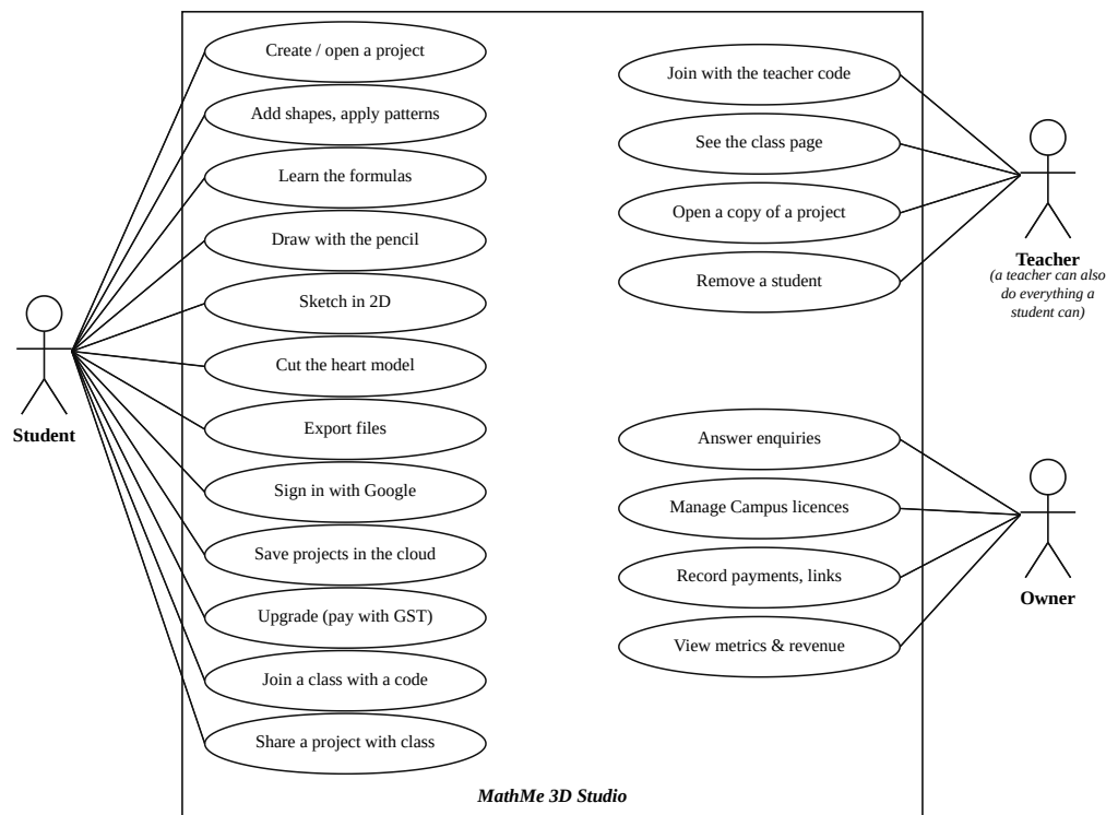
Figure 3.5: Use case diagram
