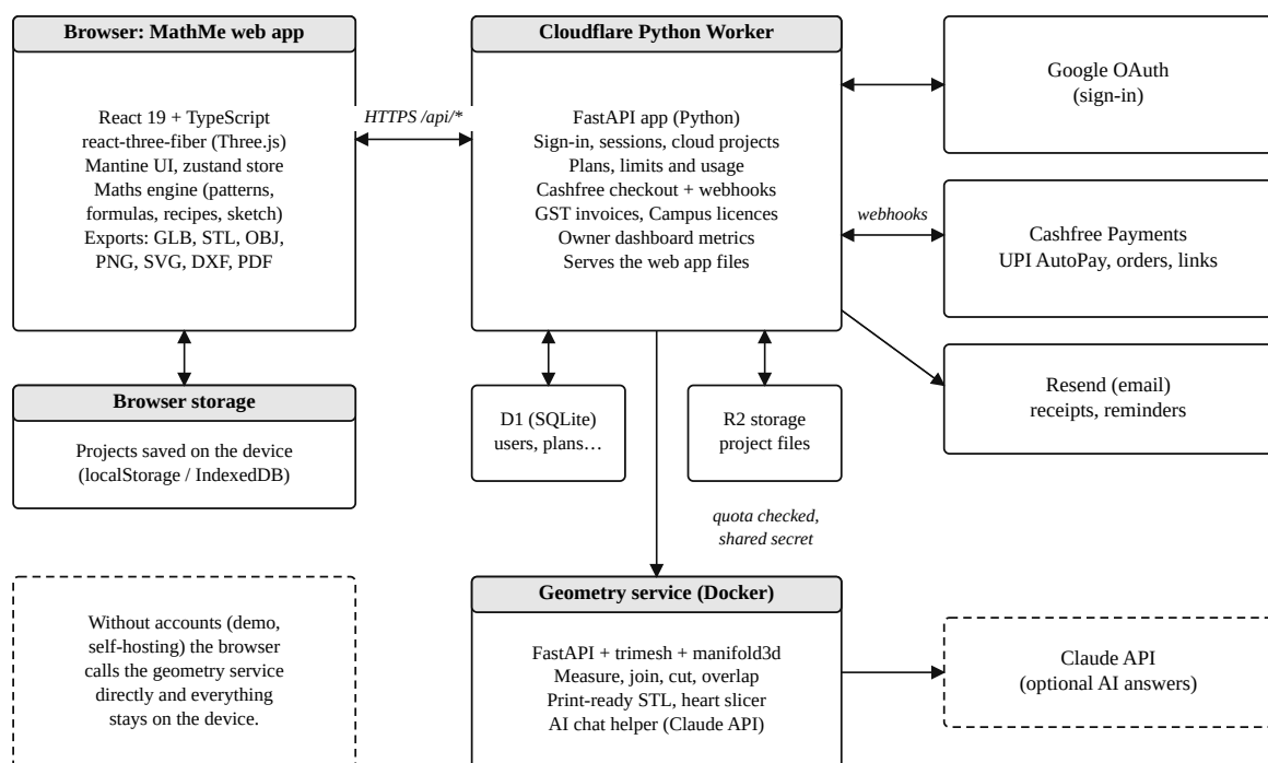
Figure 3.1: System architecture of MathMe
