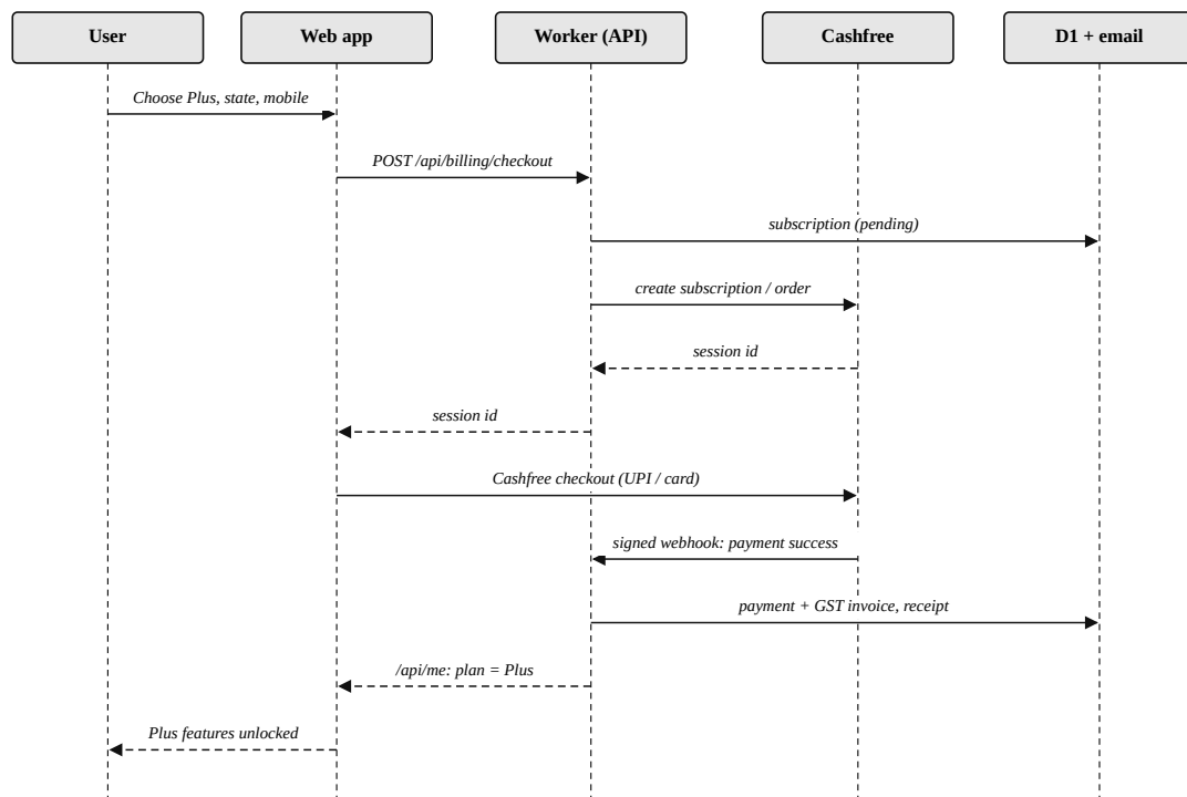
Figure 3.25: Sequence diagram of a Plus checkout
