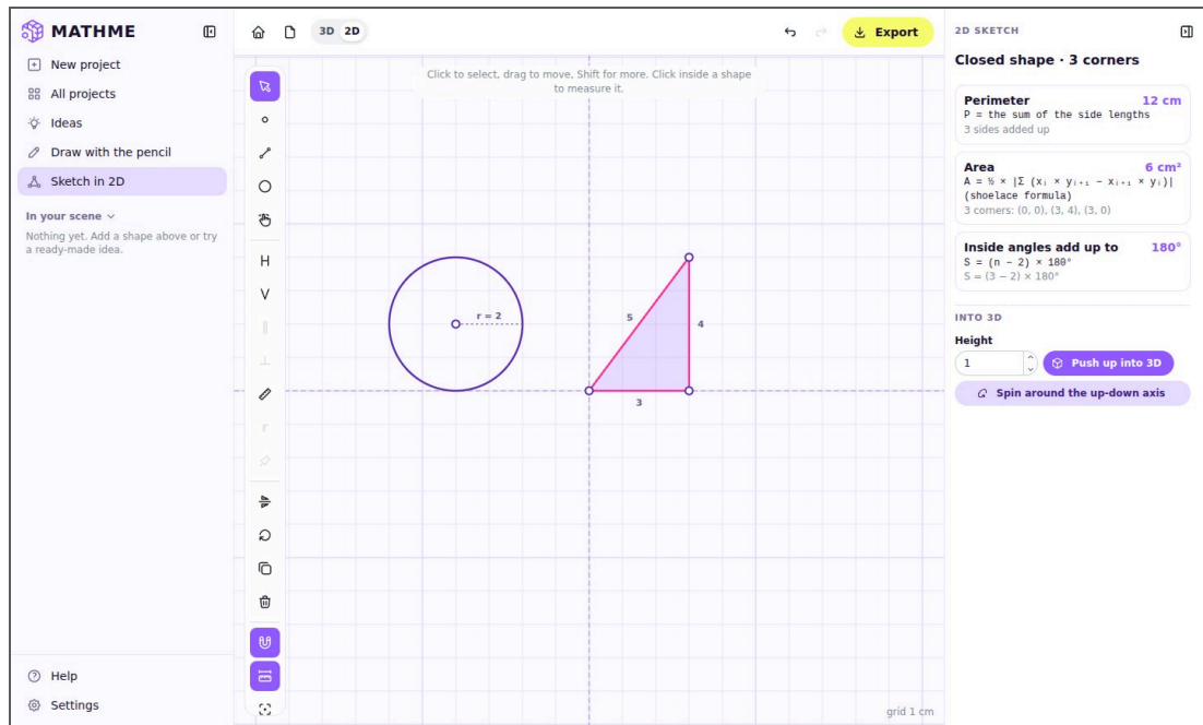
Figure 3.18: The 2D sketch board: a 3-4-5 triangle (area 6 cm 2 ) and a circle of radius 2
