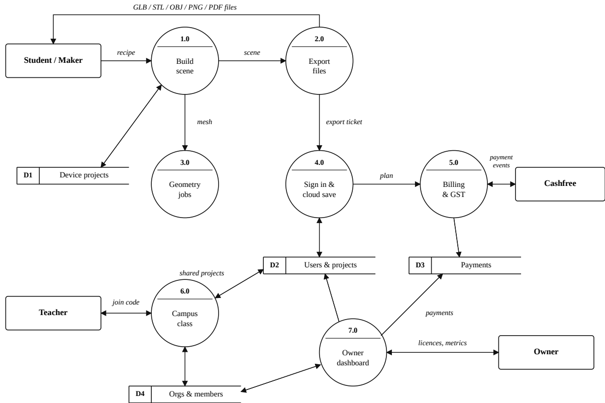
Figure 3.3: Level 1 data flow diagram
