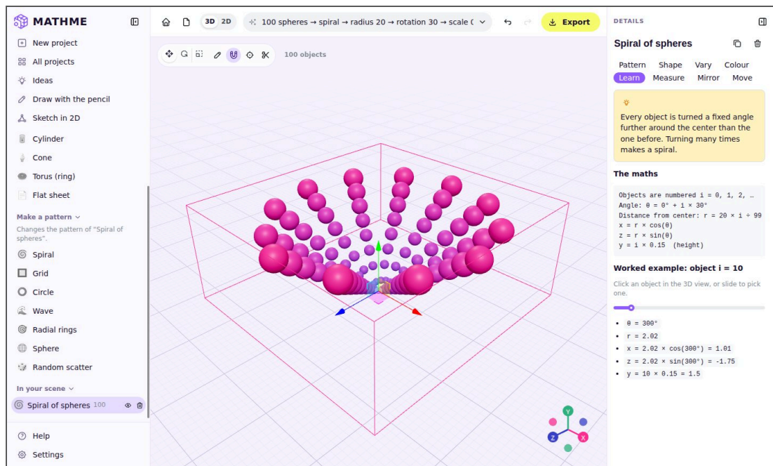
Figure 3.10: The Learn panel with the spiral formulas and a worked example
