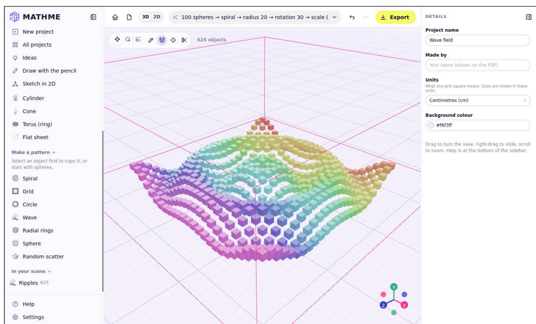
Figure 3.13: The “Wave field” idea: 625 cubes rising and falling as y = A \sin(\text{distance})
