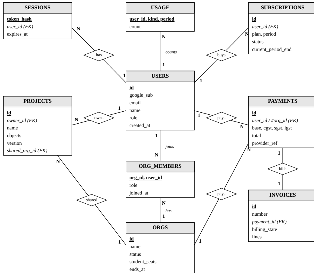
Figure 3.4: Entity-relationship diagram of the account database
