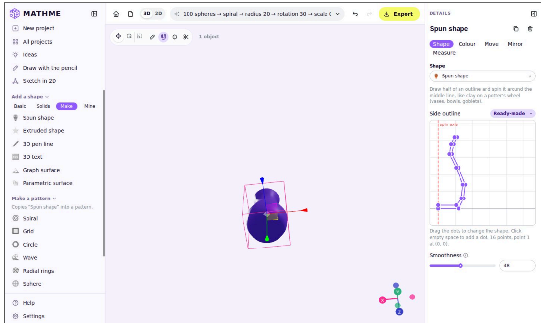
Figure 3.14: A spun (lathe) shape and its editable side outline
