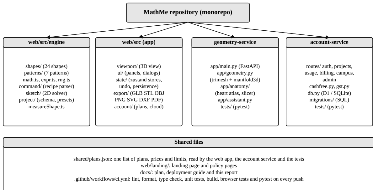
Figure 3.6: Module structure of the MathMe repository
