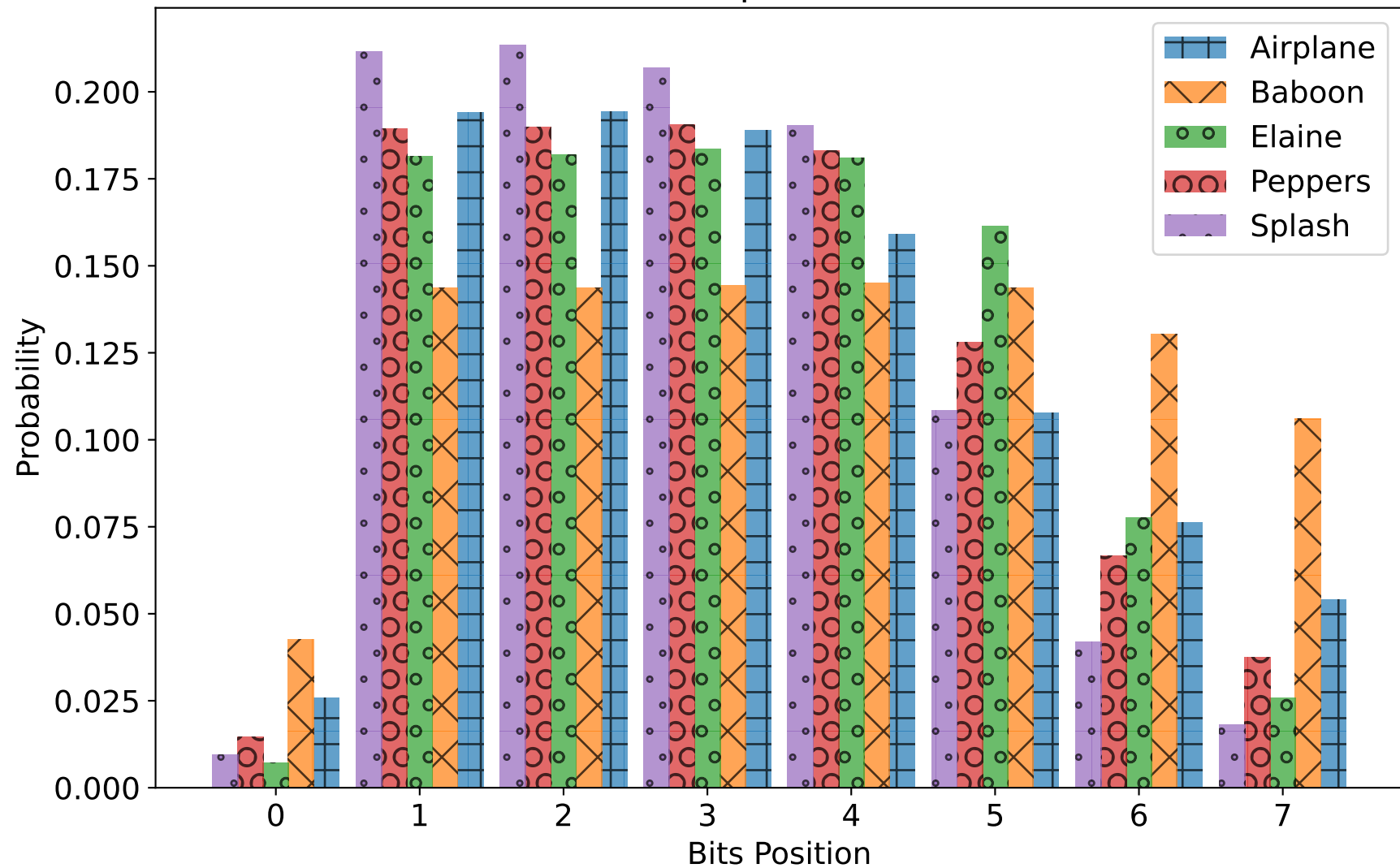
Output PMF
