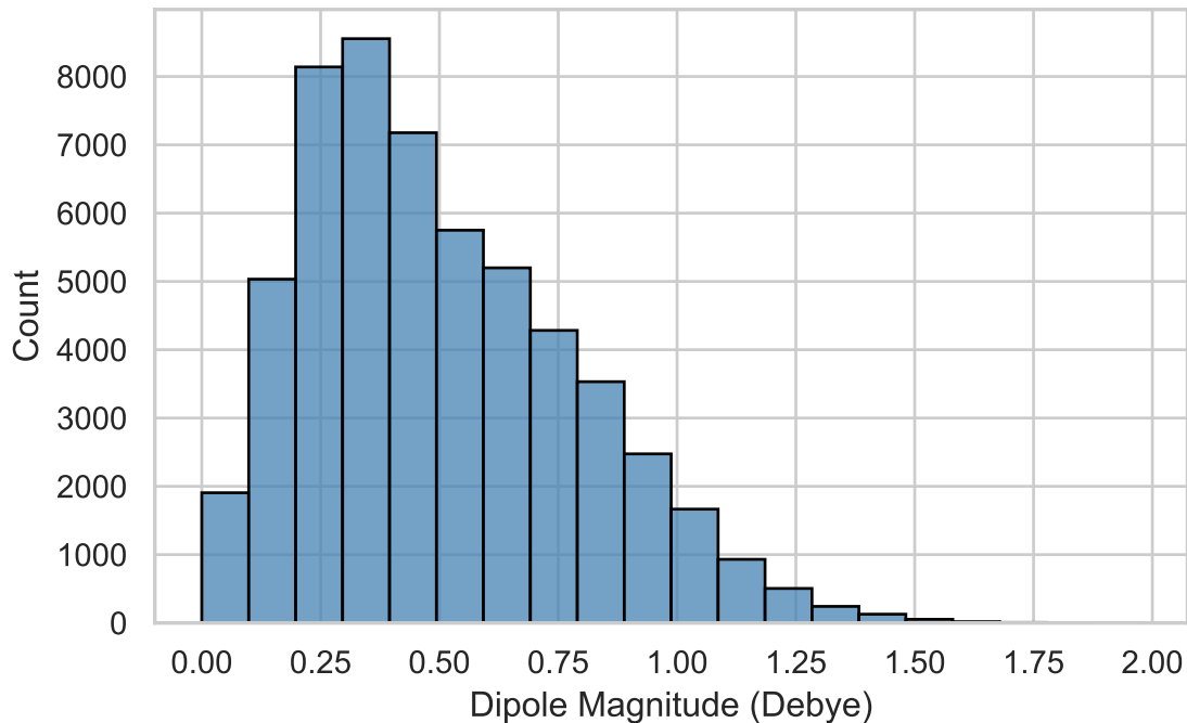
Dipole Histogram: data/mini_10_conf_qm7x_processed_train.h5
