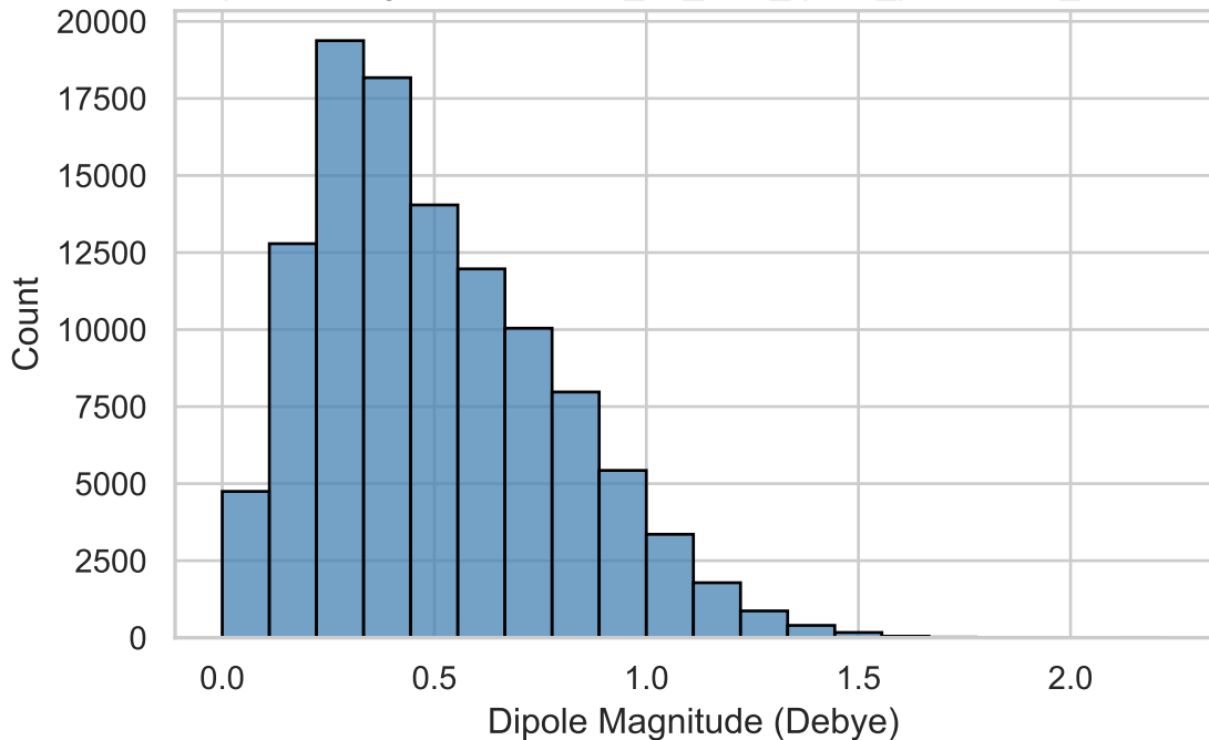
Dipole Histogram: data/mini_20_conf_qm7x_processed_train.h5
