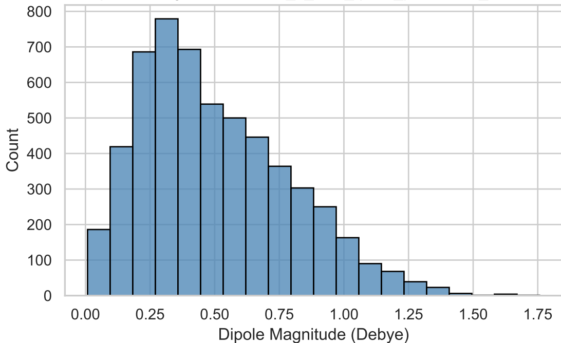
Dipole Histogram: data/mini_1_conf_qm7x_processed_train.h5
