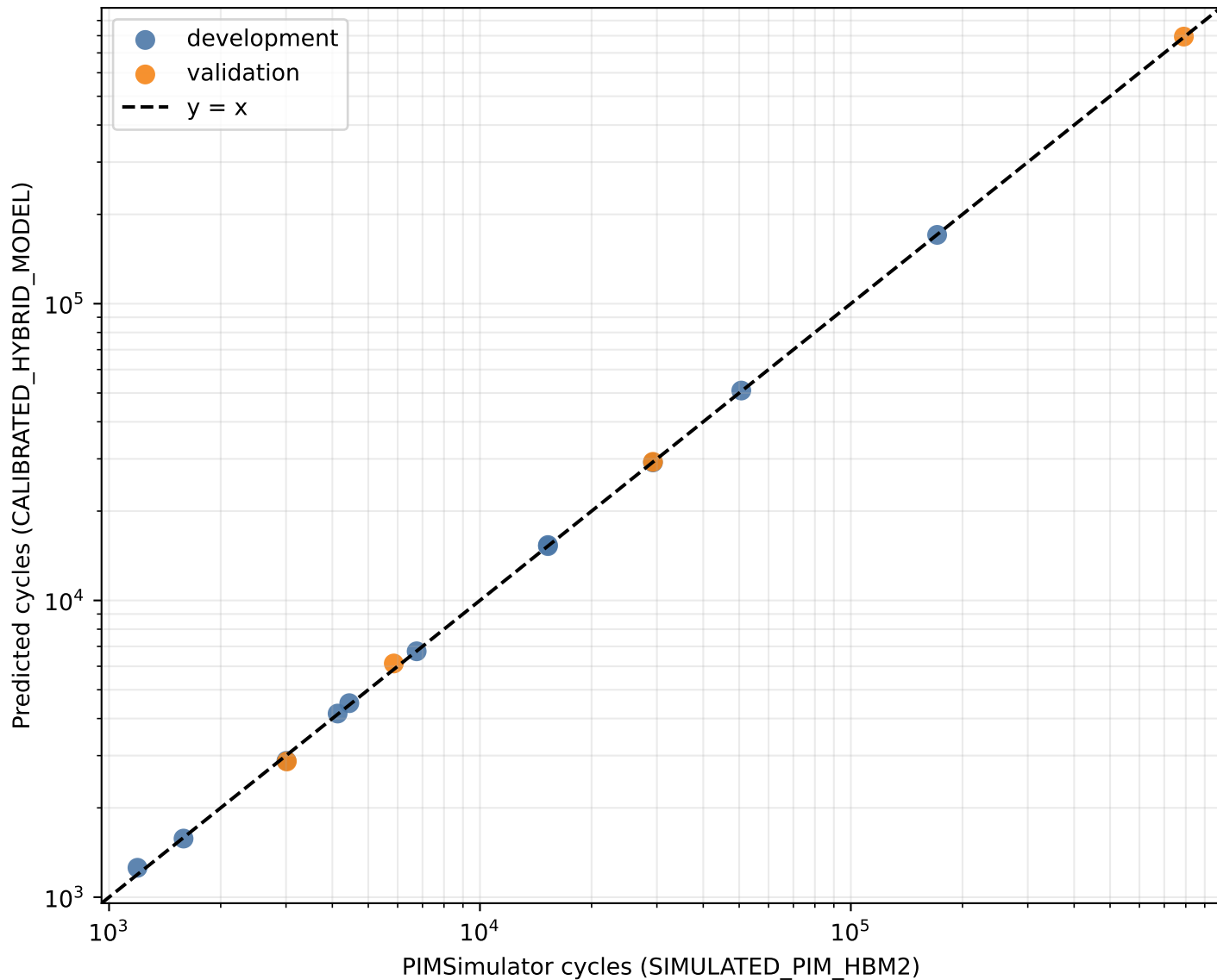
Analytical prediction versus PIMSimulator (all development and locked cases; no outliers removed)
